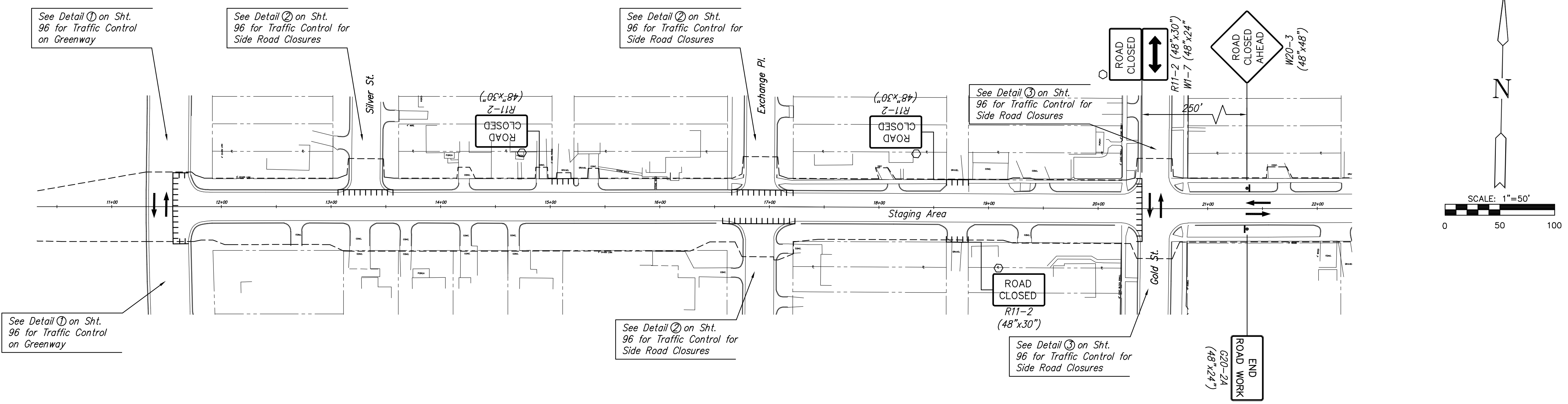
TYPICAL TRAFFIC CONTROL PLAN
