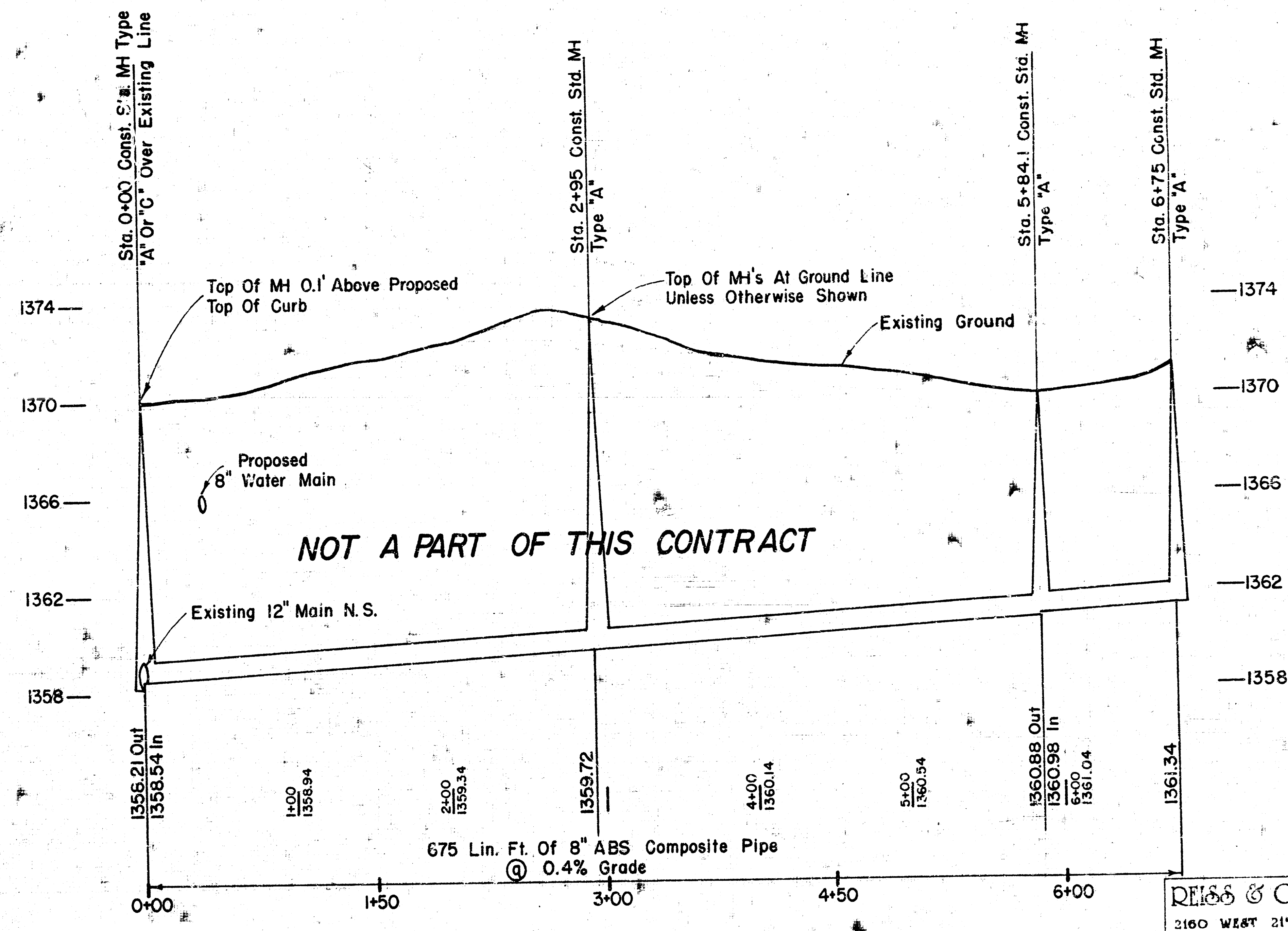
Lateral B Scale 1" = 60' Horiz. 1" = 4' Vert.
