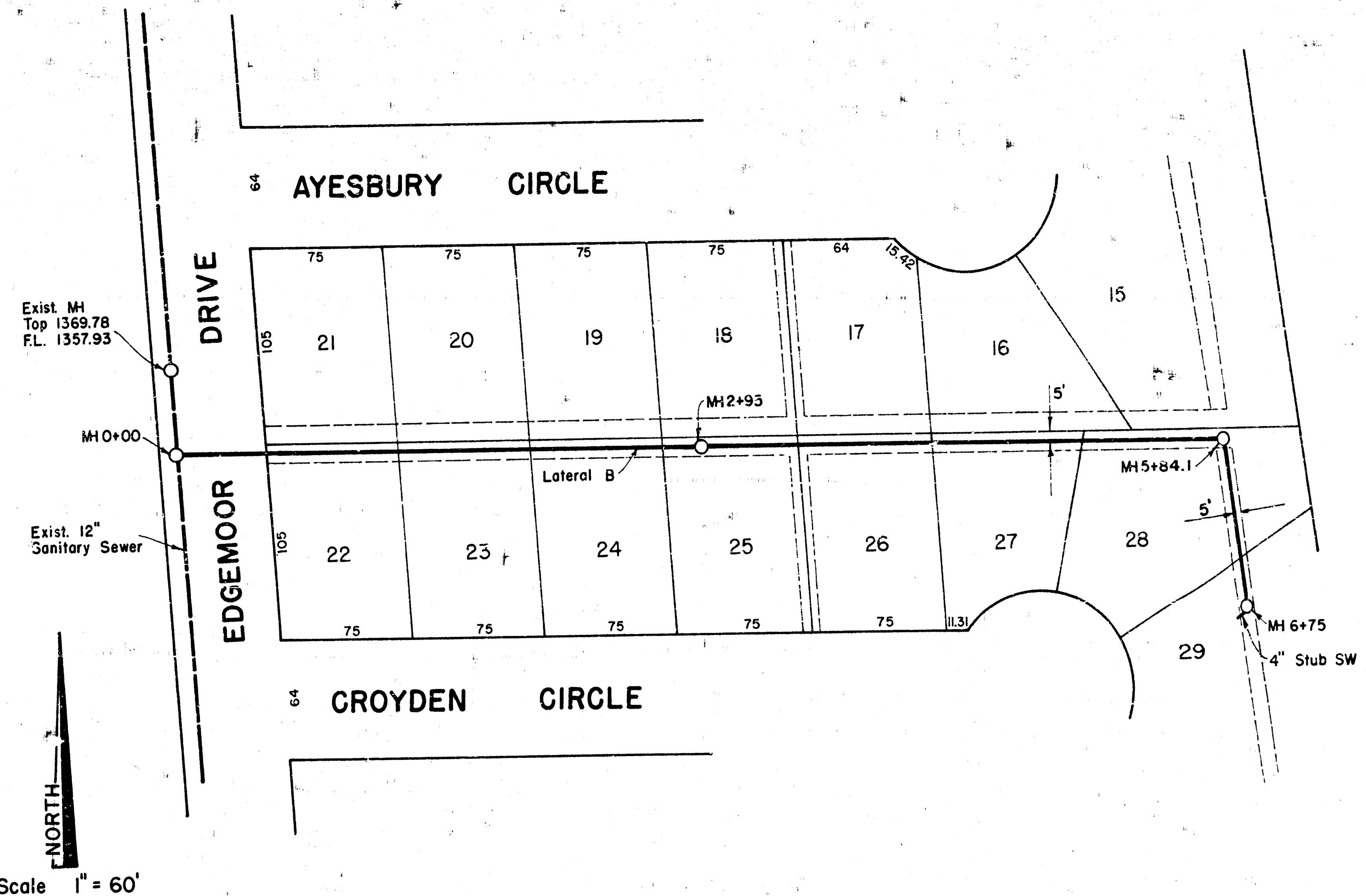
Lateral B Scale 1" = 60' Horiz. 1" = 4' Vert.
