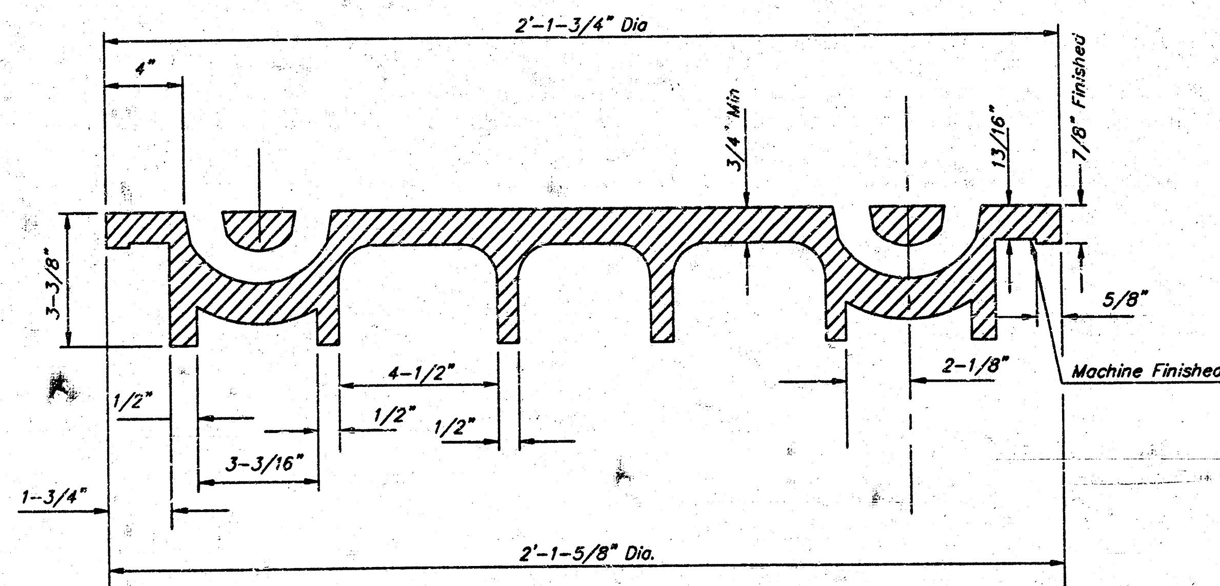
SECTION VIEW
