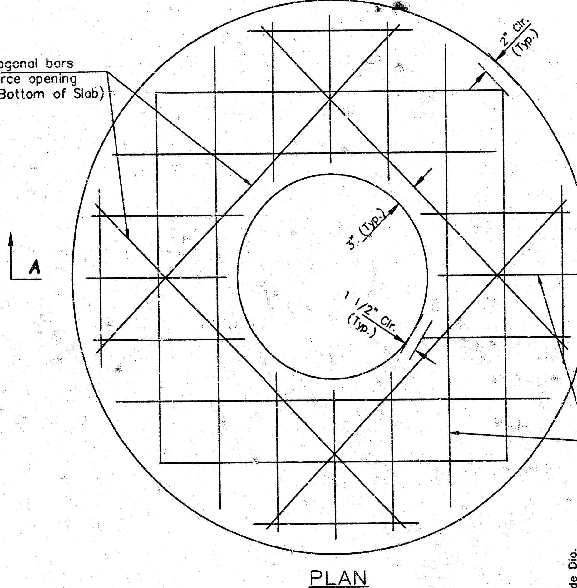
PLAN
