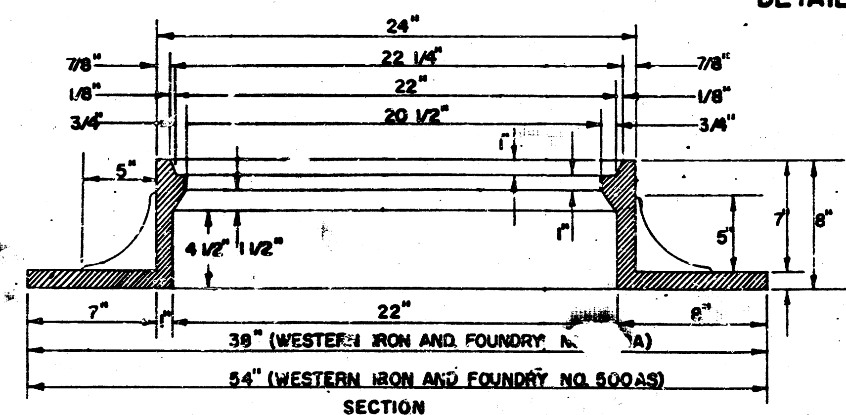
OUTSIDE CIRCUMFERENCE OF COVER AND THE INNER FACE AND SEAT OF RING TO BE MACHINE FIT.
