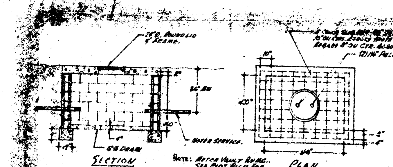
WATER METER VAULT DETAIL SCALE 1/8"=1'-0"
