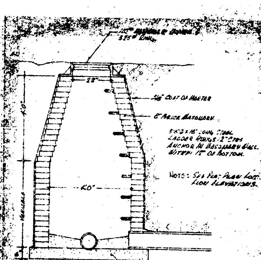
MANHOLE DETAIL NO SCALE
