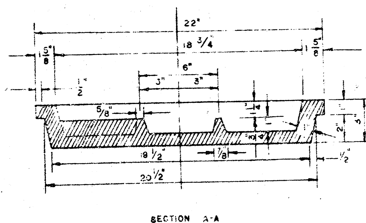
MANHOLE COVER WEIGHT 110 LBS.
