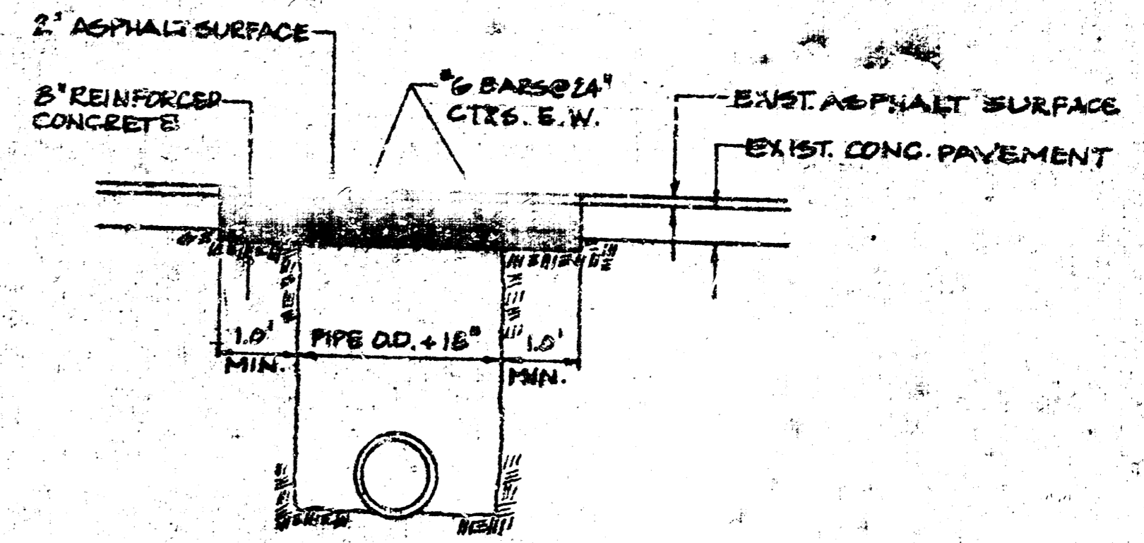
PAVEMENT REPLACEMENT DETAIL NO SCALE
