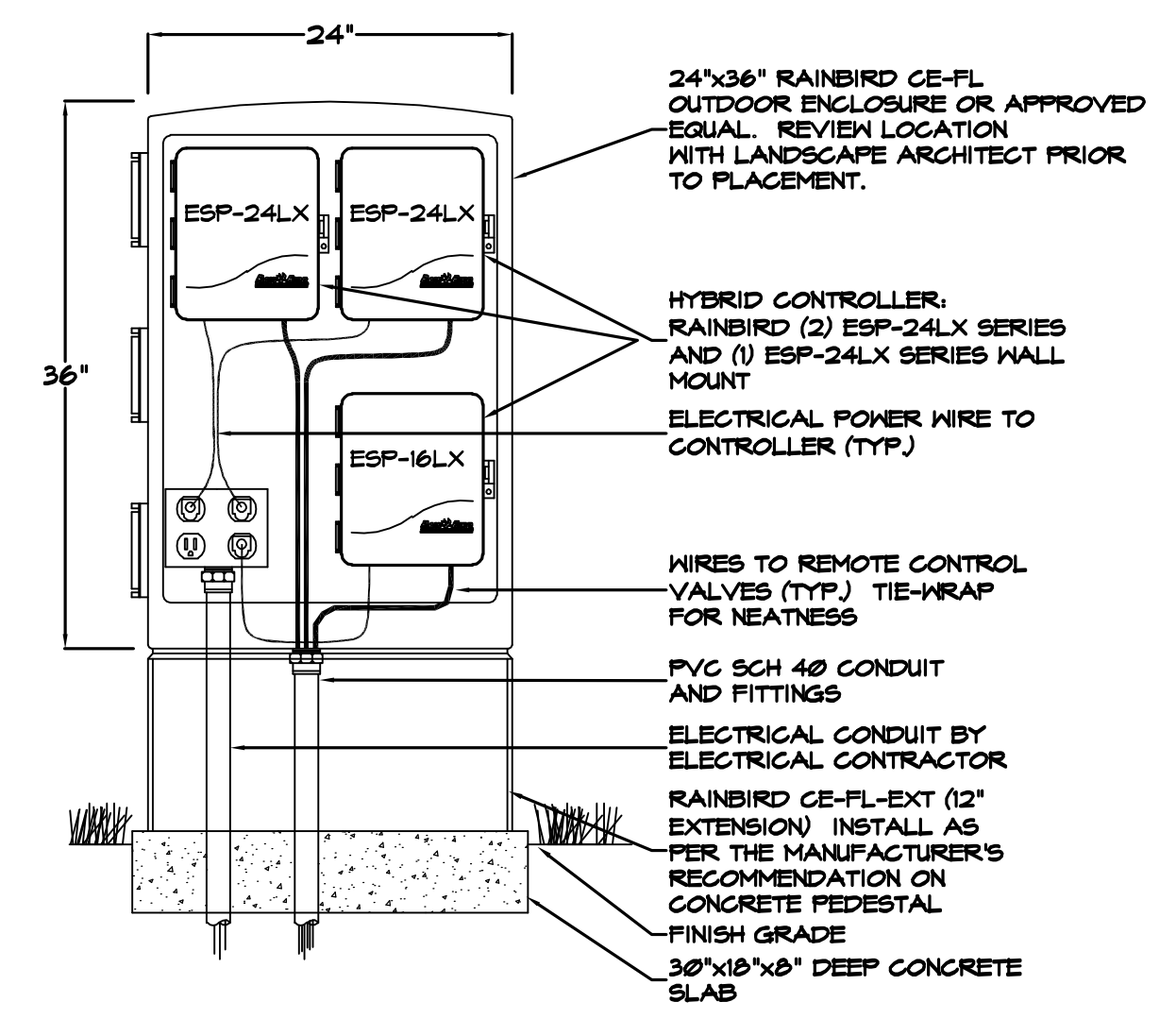
IRRIGATION CONTROLLER PEDESTAL NO SCALE
