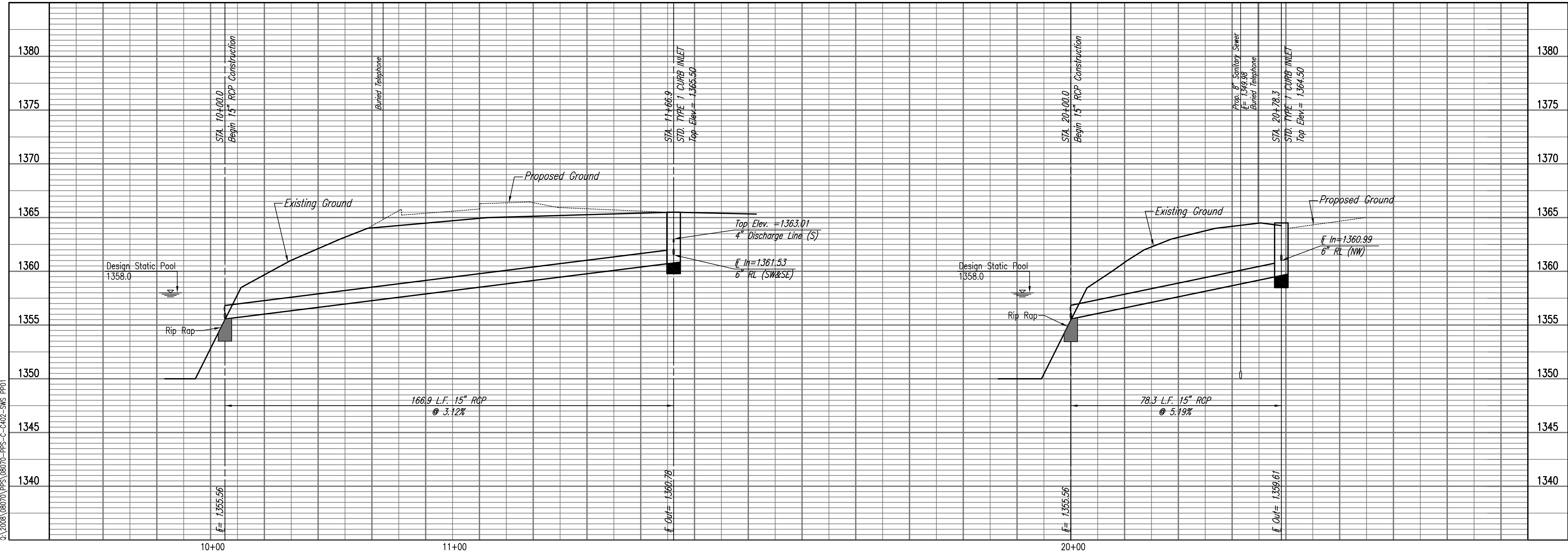
STORM WATER SEWER LINE NO. 1
