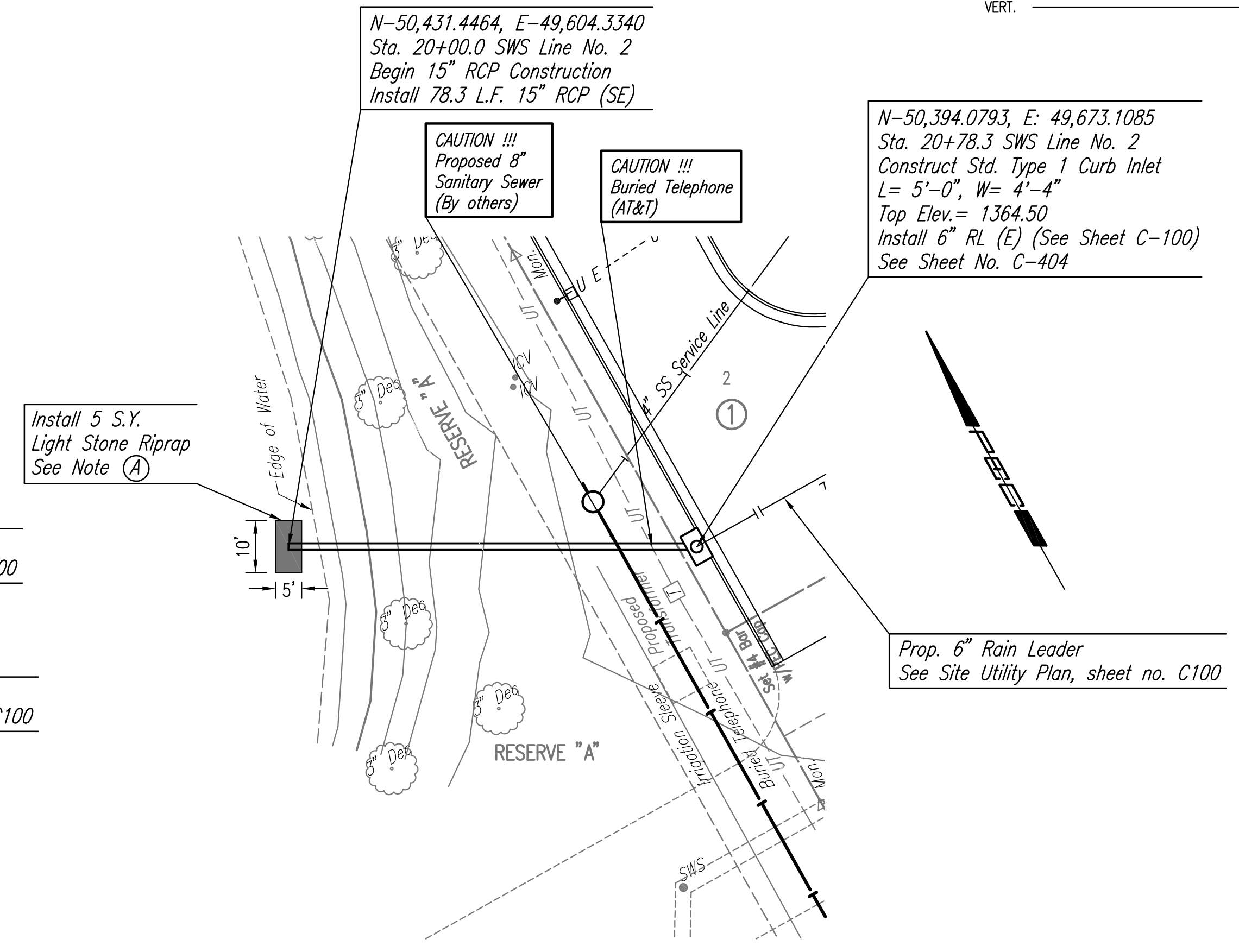
STORM WATER SEWER LINE NO. 2
