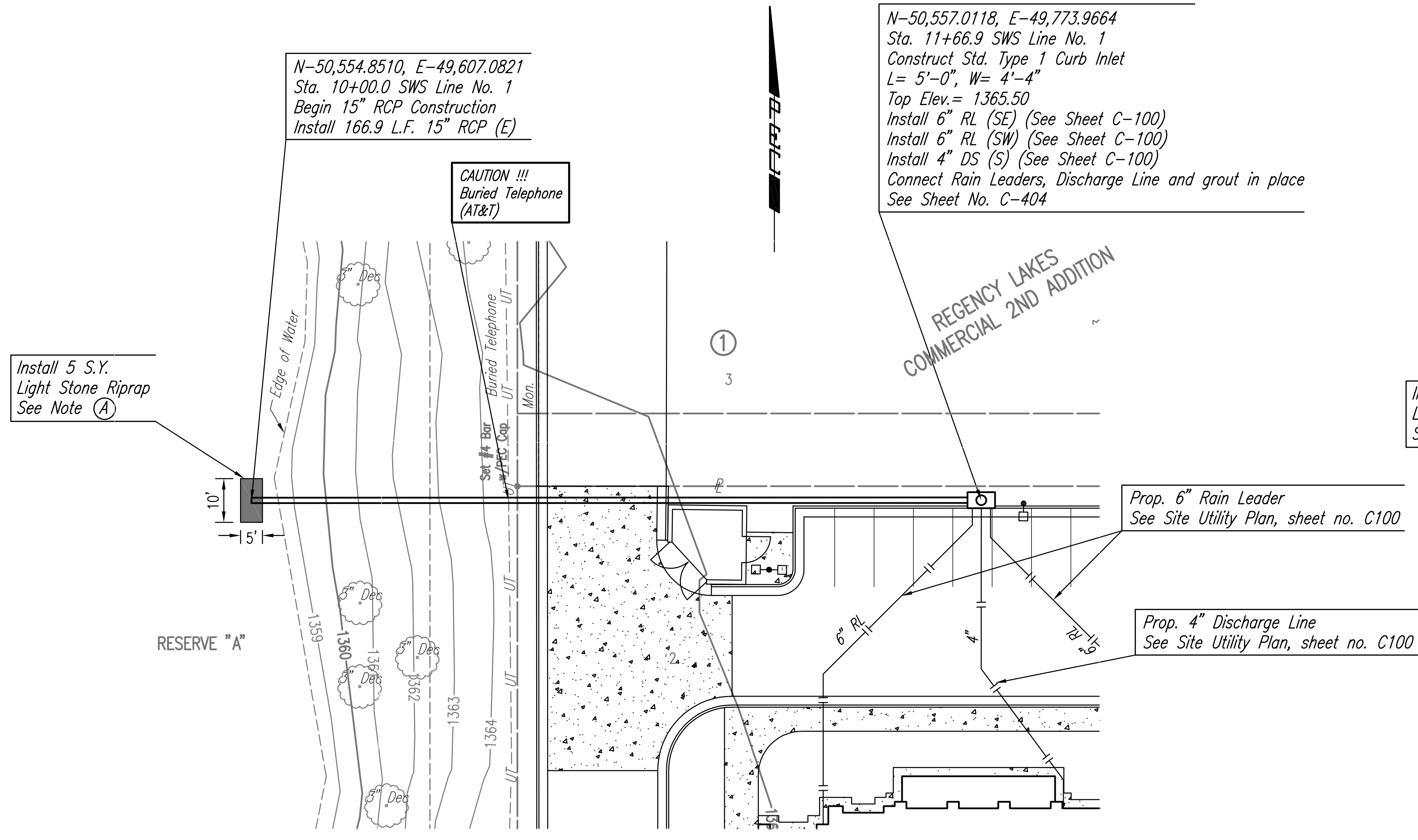
STORM WATER SEWER LINE NO. 1
