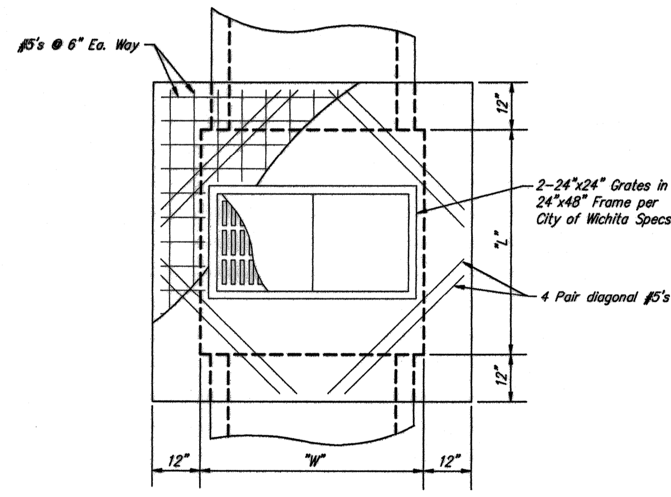
PLAN VIEW TYPE "A" INLET SCALE: 1/2"=1'-0"
