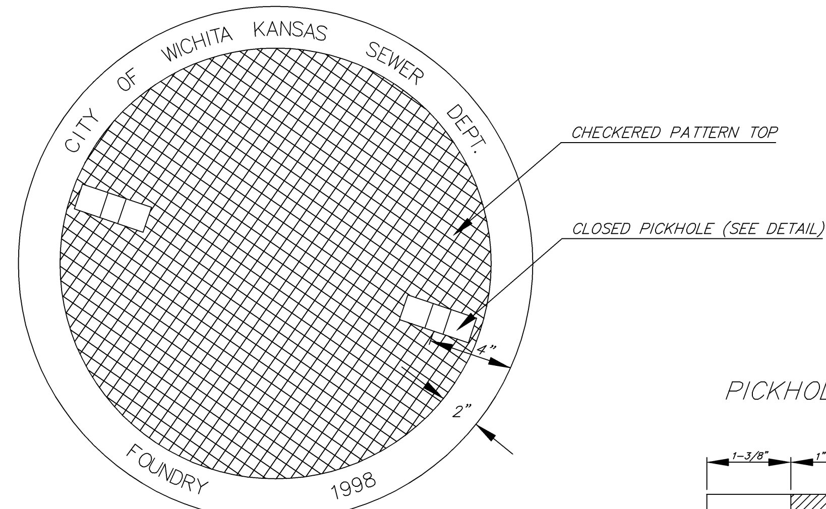
TOP VIEW
