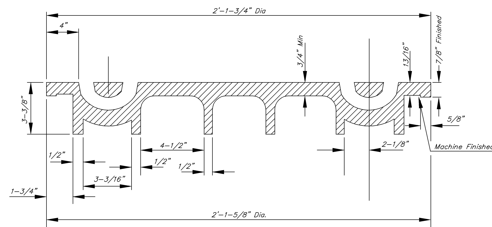
SECTION VIEW
