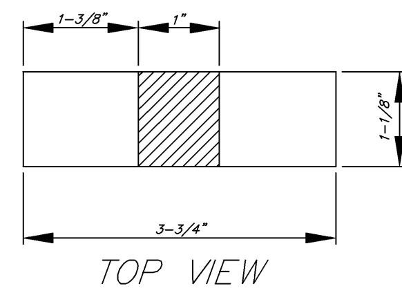
PICKHOLE DETAIL
