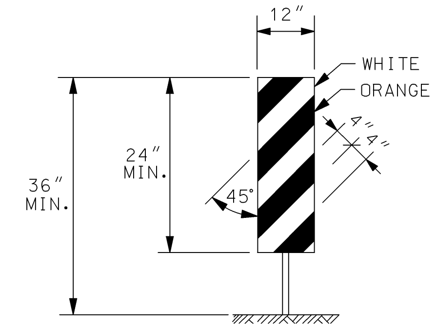
VERTICAL PANEL
