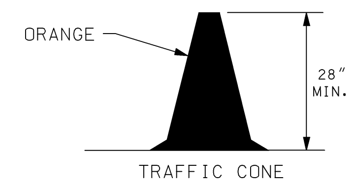
TRAFFIC CONE
