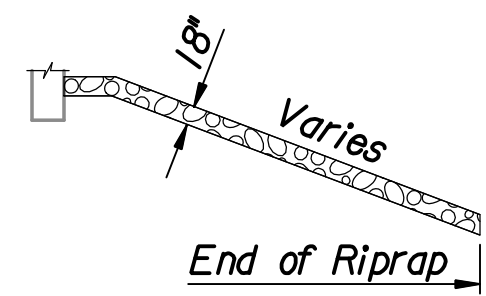
TYPICAL RIPRAP SECTION
