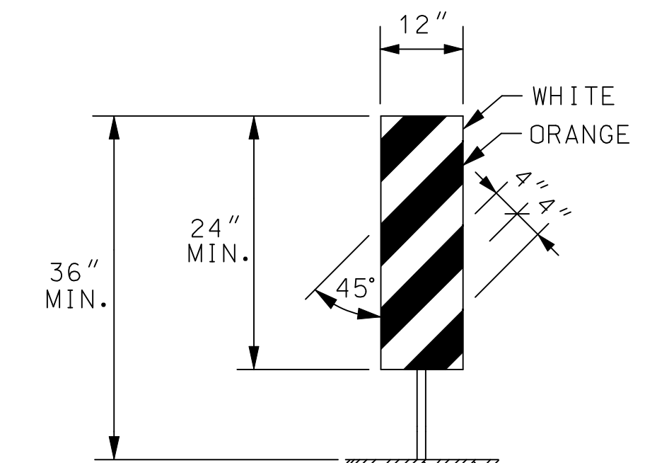
VERTICAL PANEL
