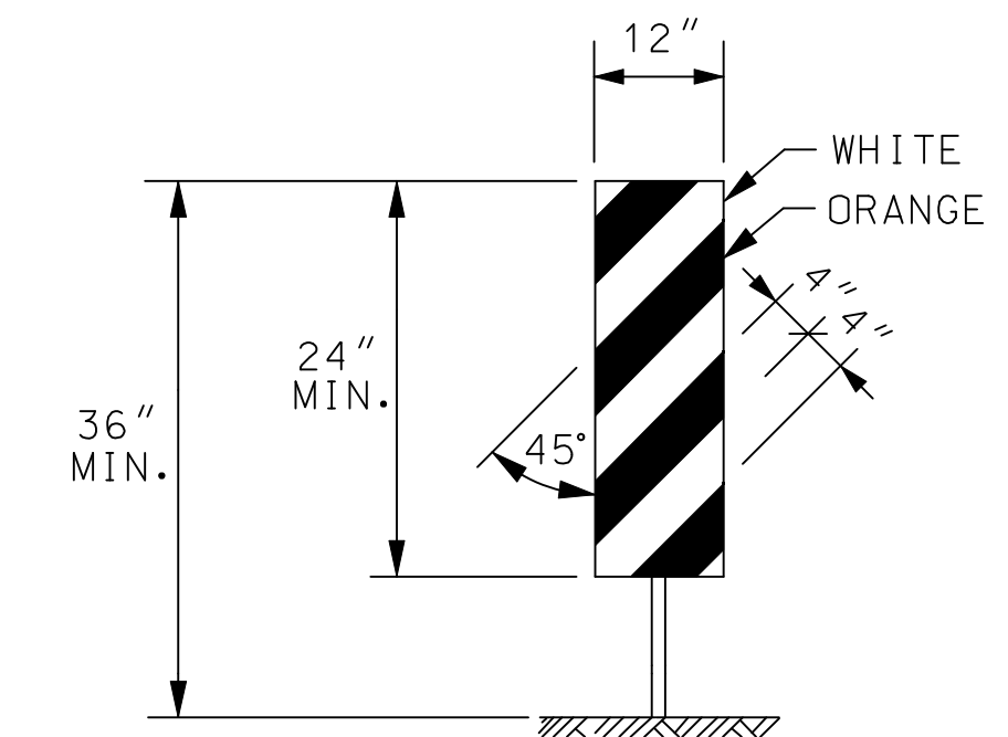
VERTICAL PANEL
