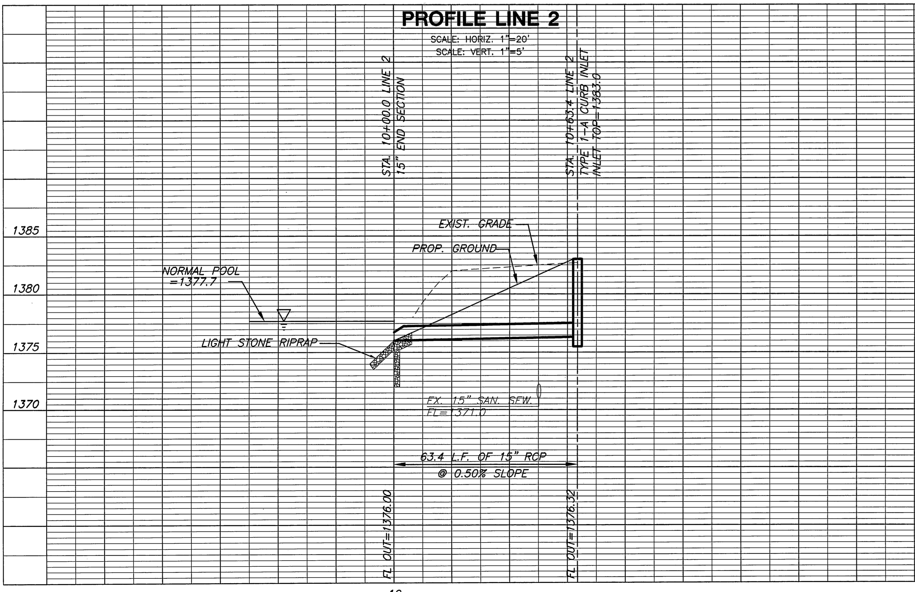
PROFILE LINE 2
