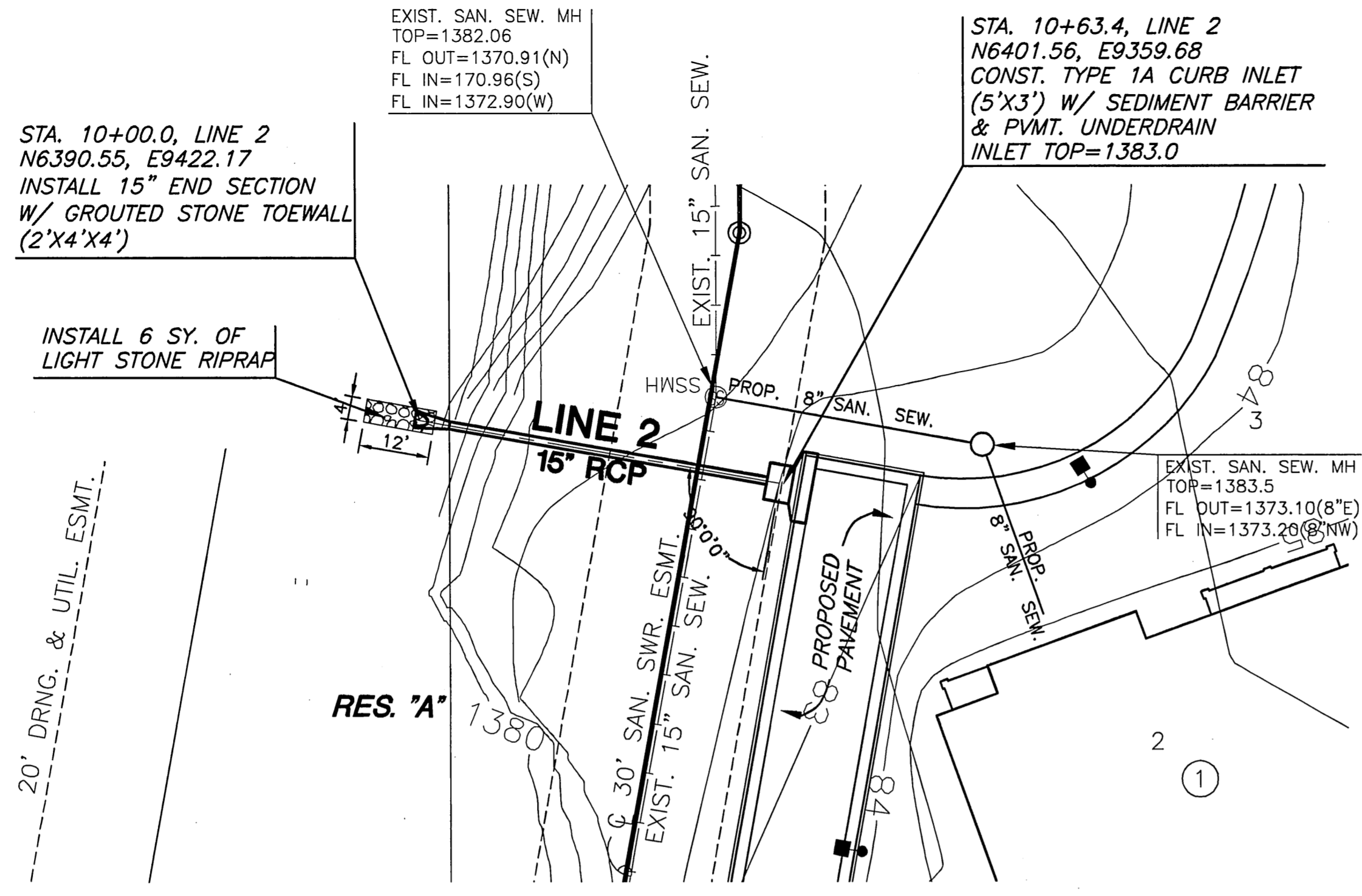
PLAN LINE 2
