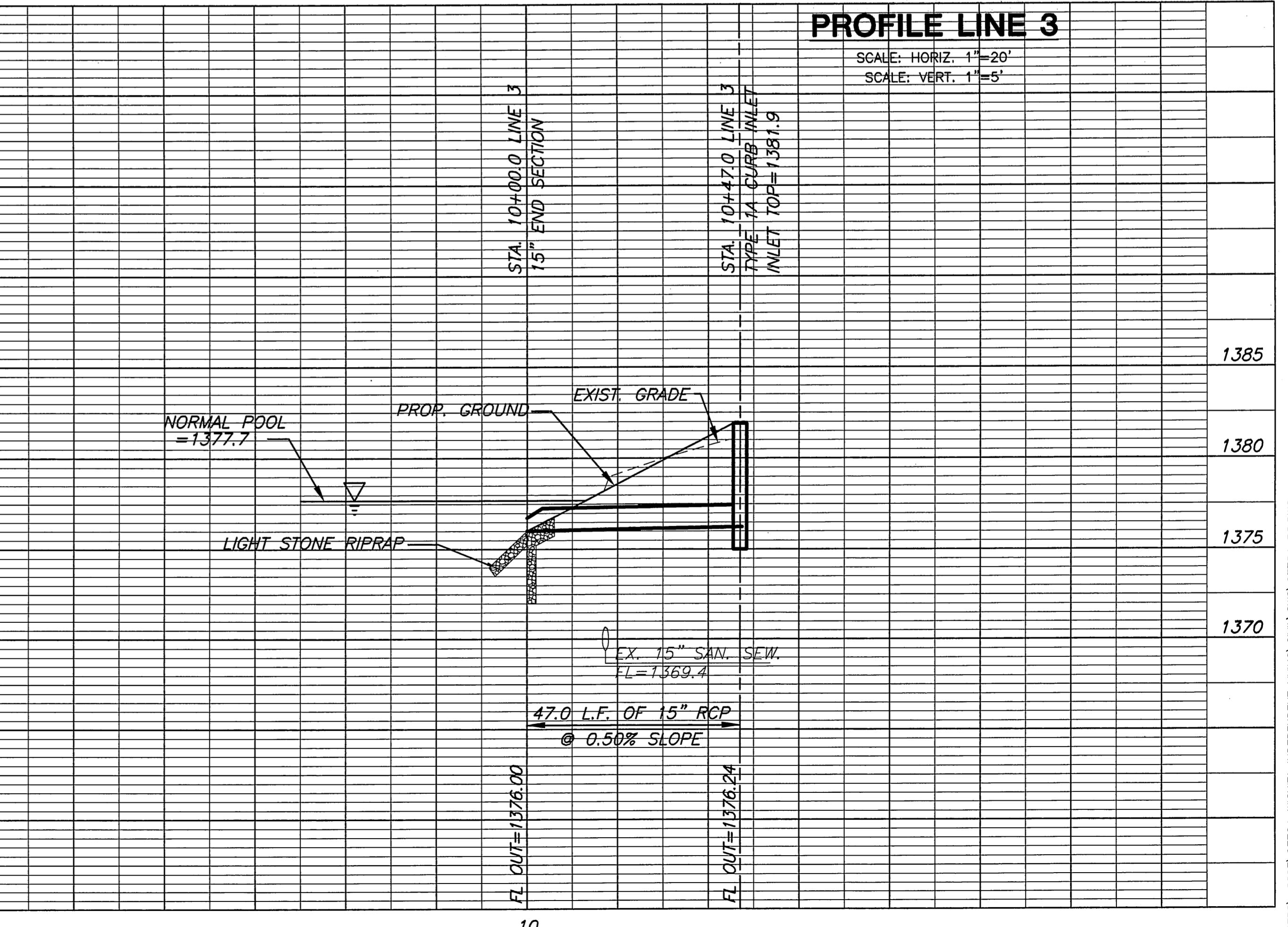
PROFILE LINE 3
