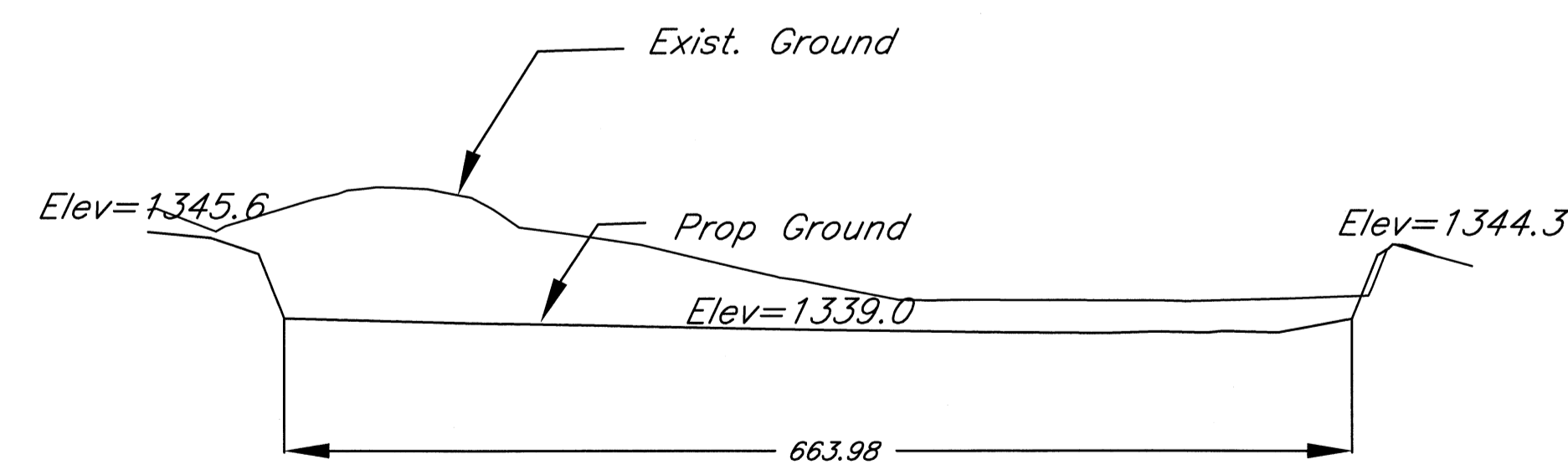
SECTION B-B
