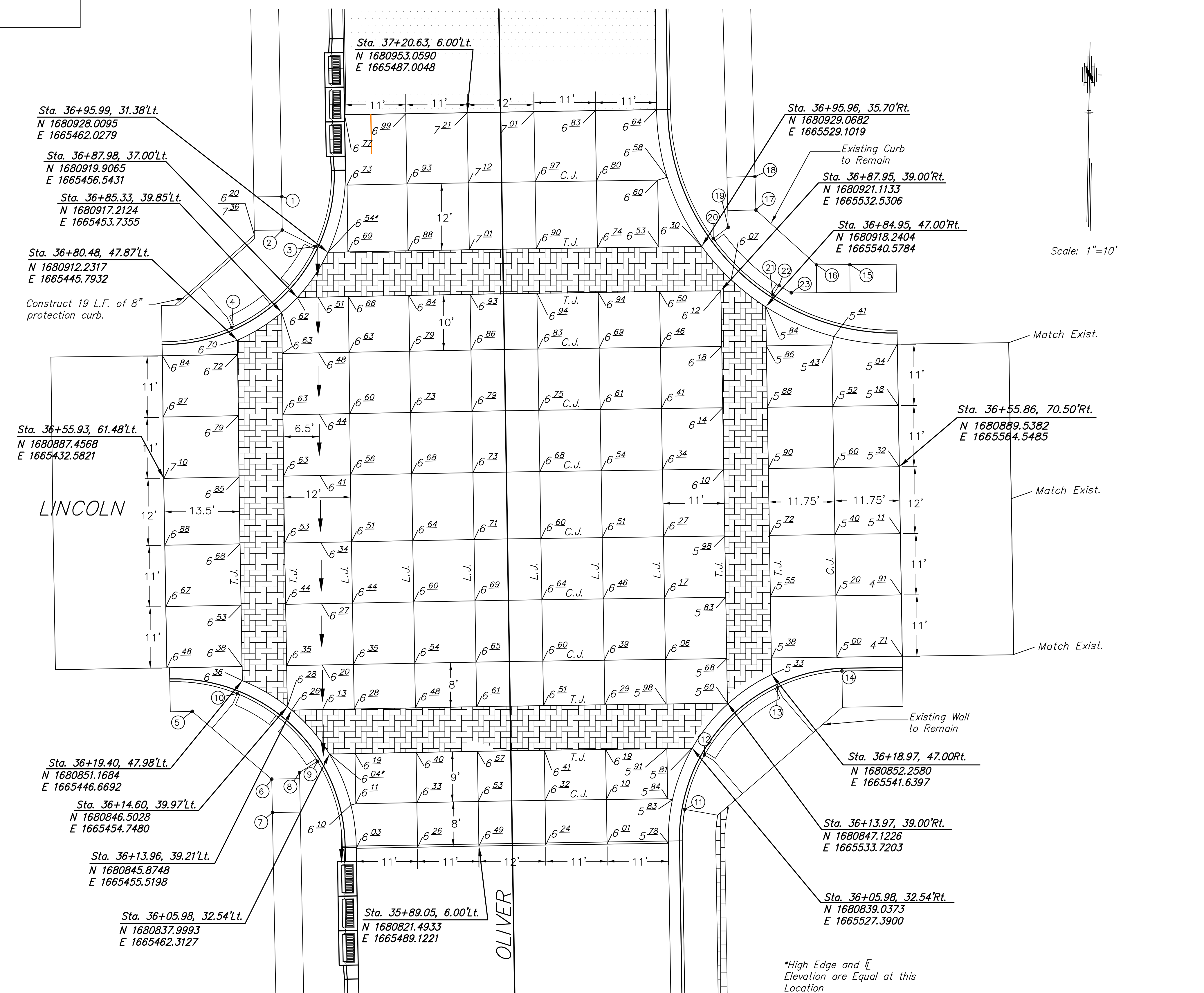
INTERSECTION JOINT PATTERN PLAN
