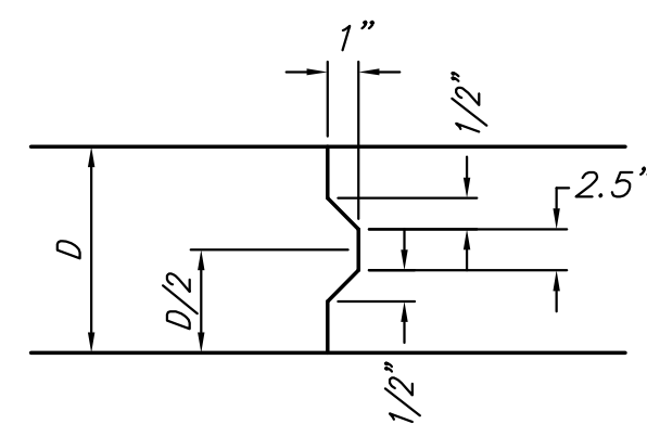
KEYWAY DETAIL
