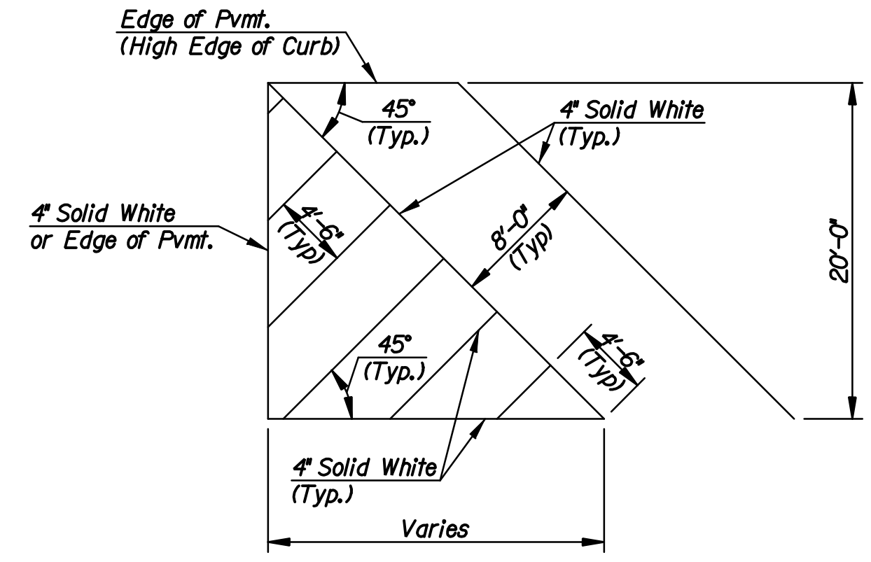
PARKING DETAIL
