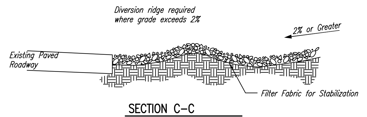
SECTION C-C
