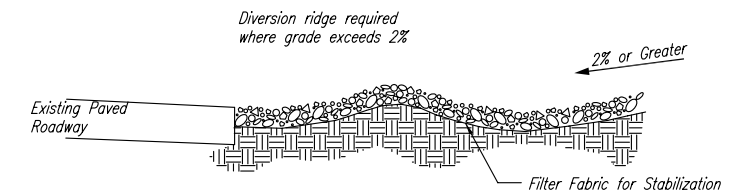
SECTION C-C
