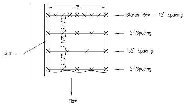
BACK OF CURB PROTECTION DETAIL
