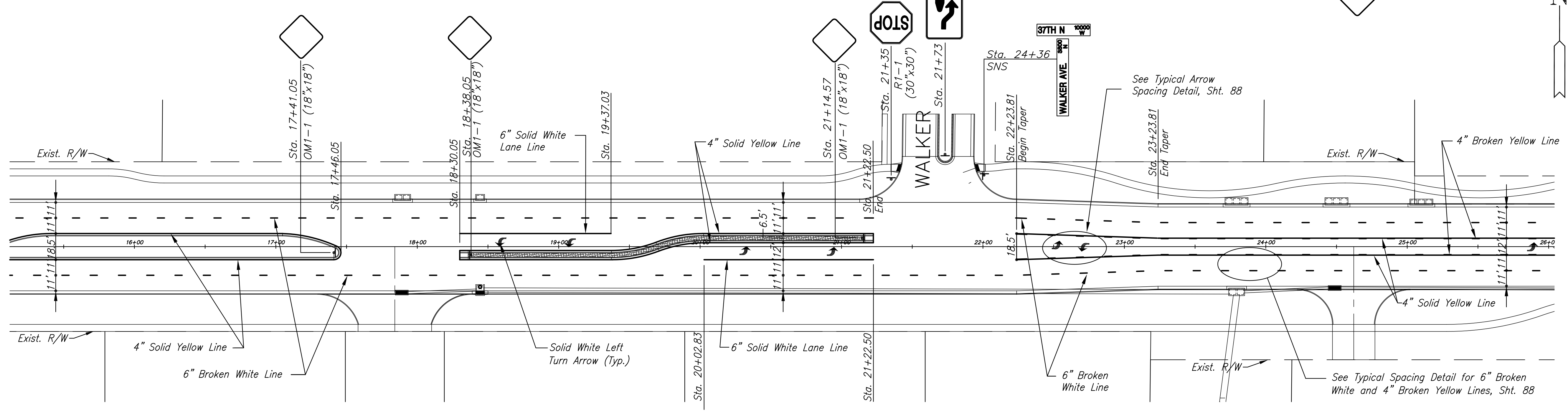
37TH STREET - PLAN
