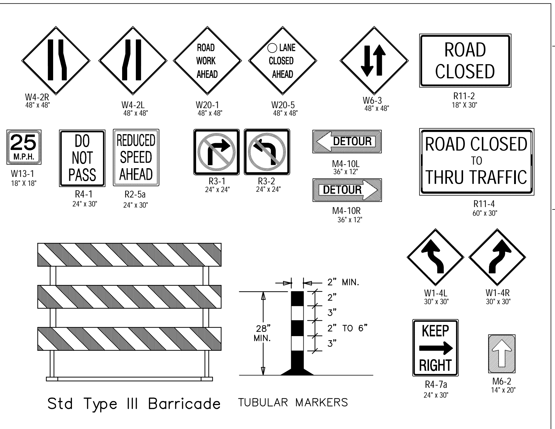
STANDARD CONSTRUCTION SIGNS AND CHANNELIZING DEVICES
