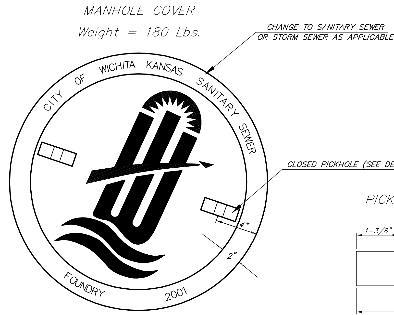
TOP VIEW
