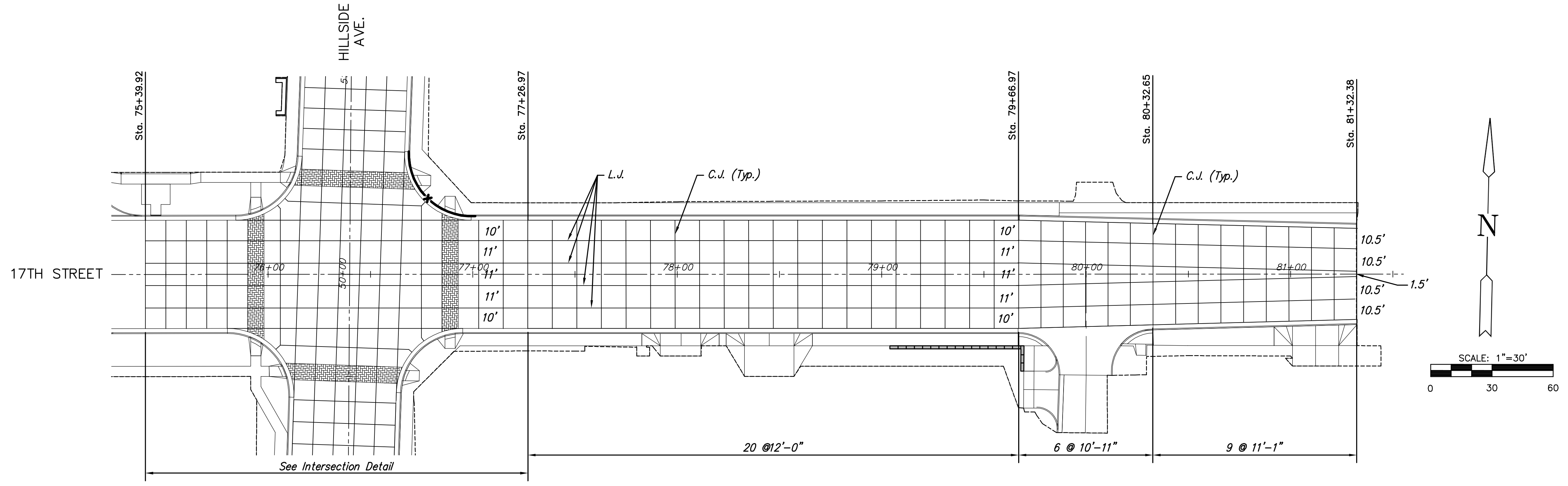
17TH STREET Sta. 75+39.92 to 81+32.18
