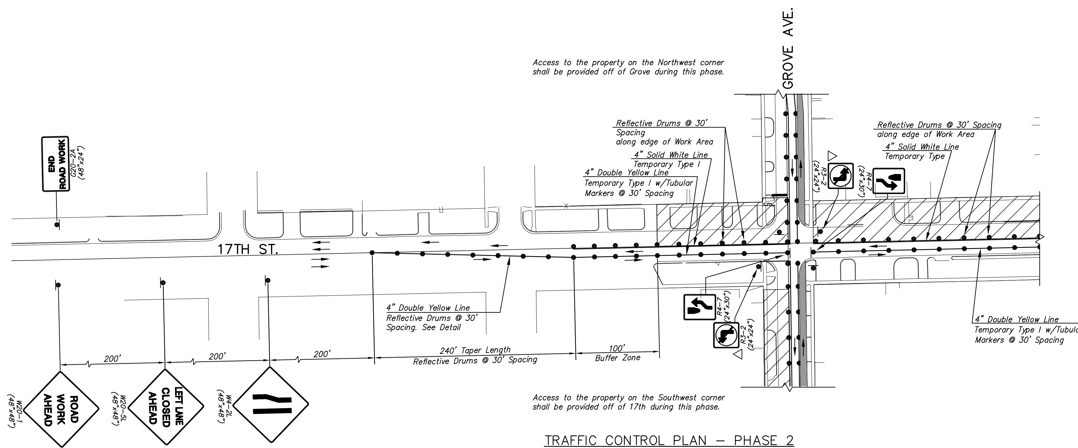
TRAFFIC CONTROL PLAN - PHASE 2
