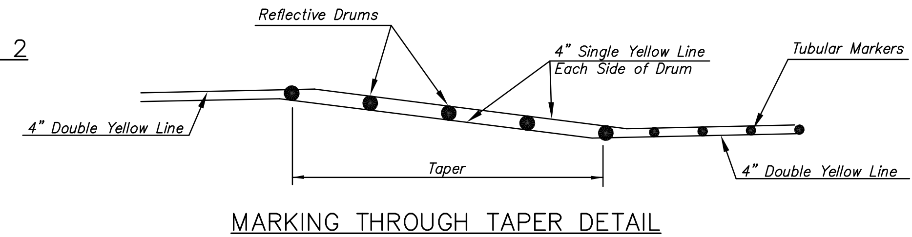
MARKING THROUGH TAPER DETAIL
