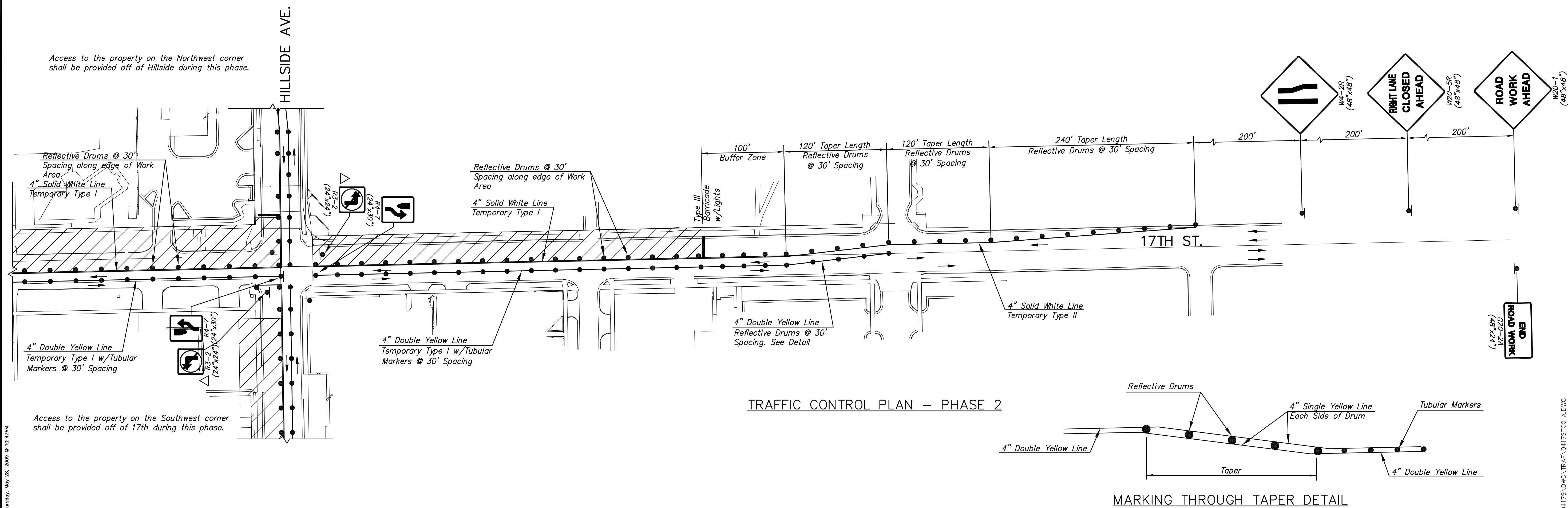
TRAFFIC CONTROL PLAN - PHASE 2
