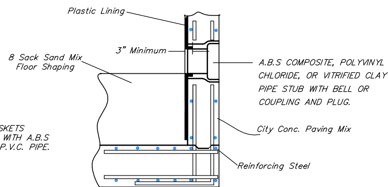
PIPE STUB DETAIL SANITARY SEWER ONLY
