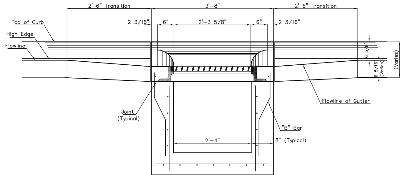
SECTION C-C
