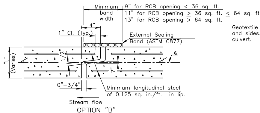
OPEN JOINT DETAIL
