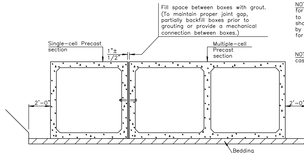
TYPICAL INSTALLATION DETAILS
