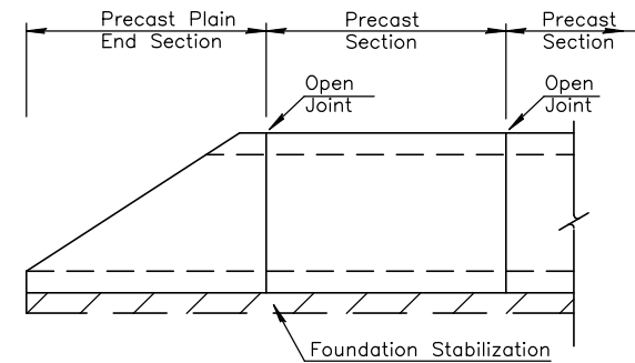
ELEVATION AT PRECAST END SECTION
