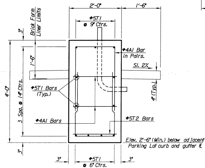
TYPICAL SECTION
