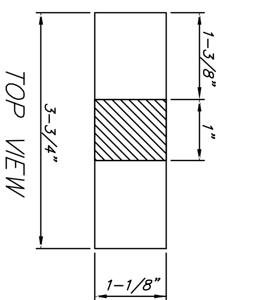
PICKHOLE DETAIL
