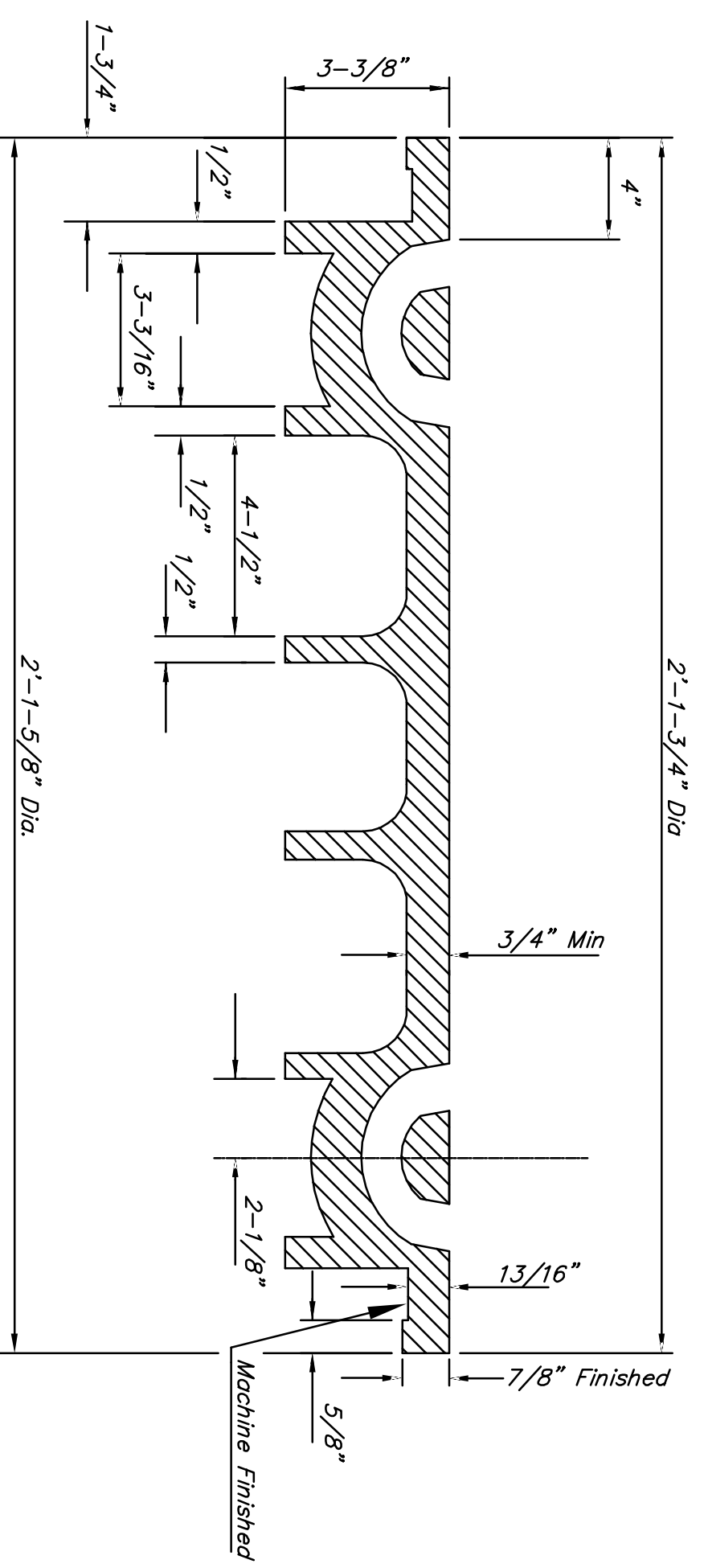
SECTION VIEW
