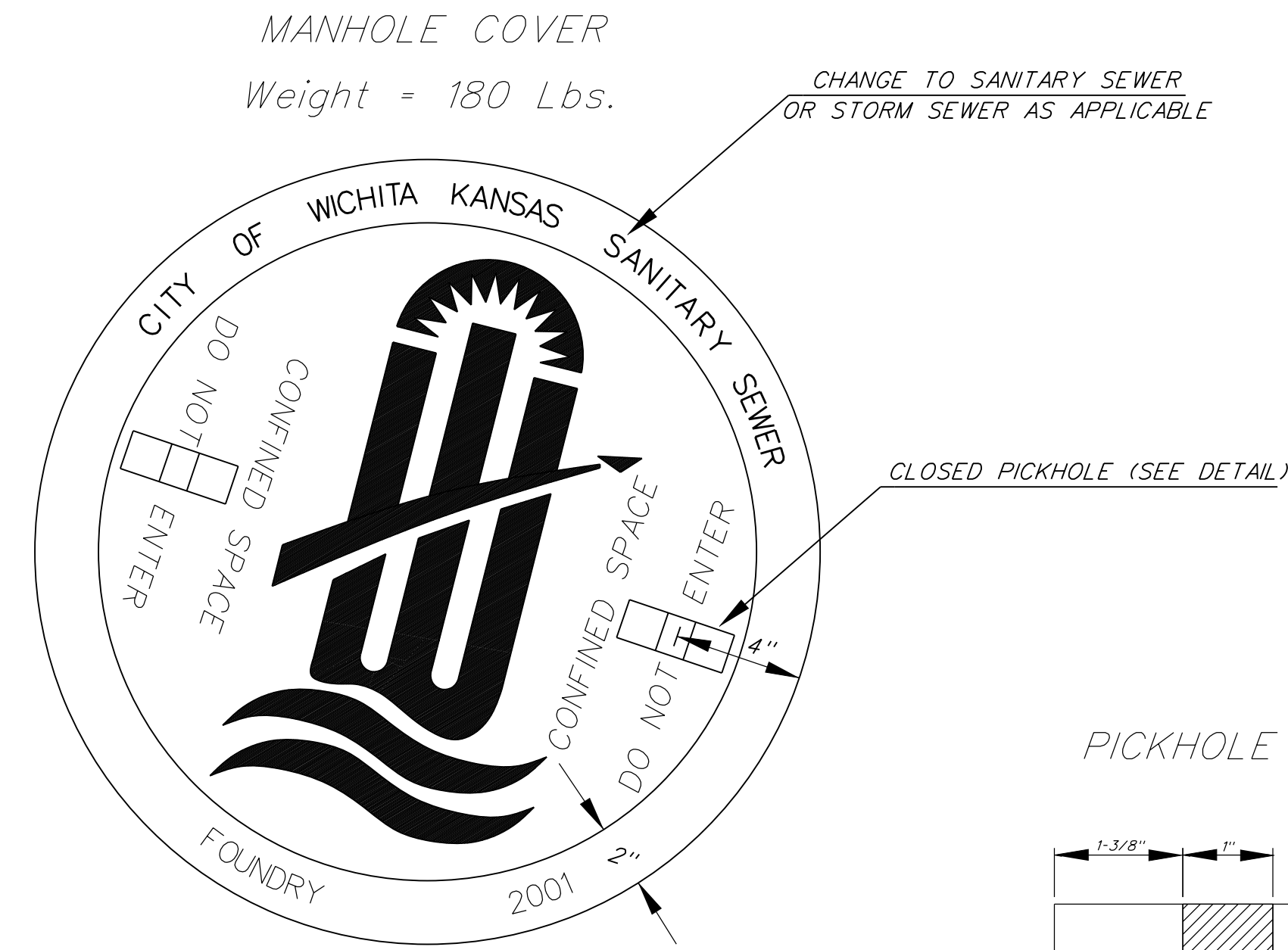
TOP VIEW
