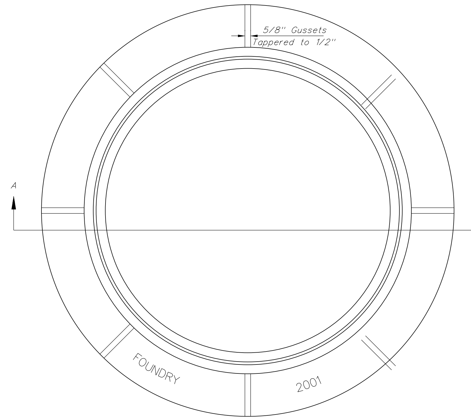
TOP VIEW
