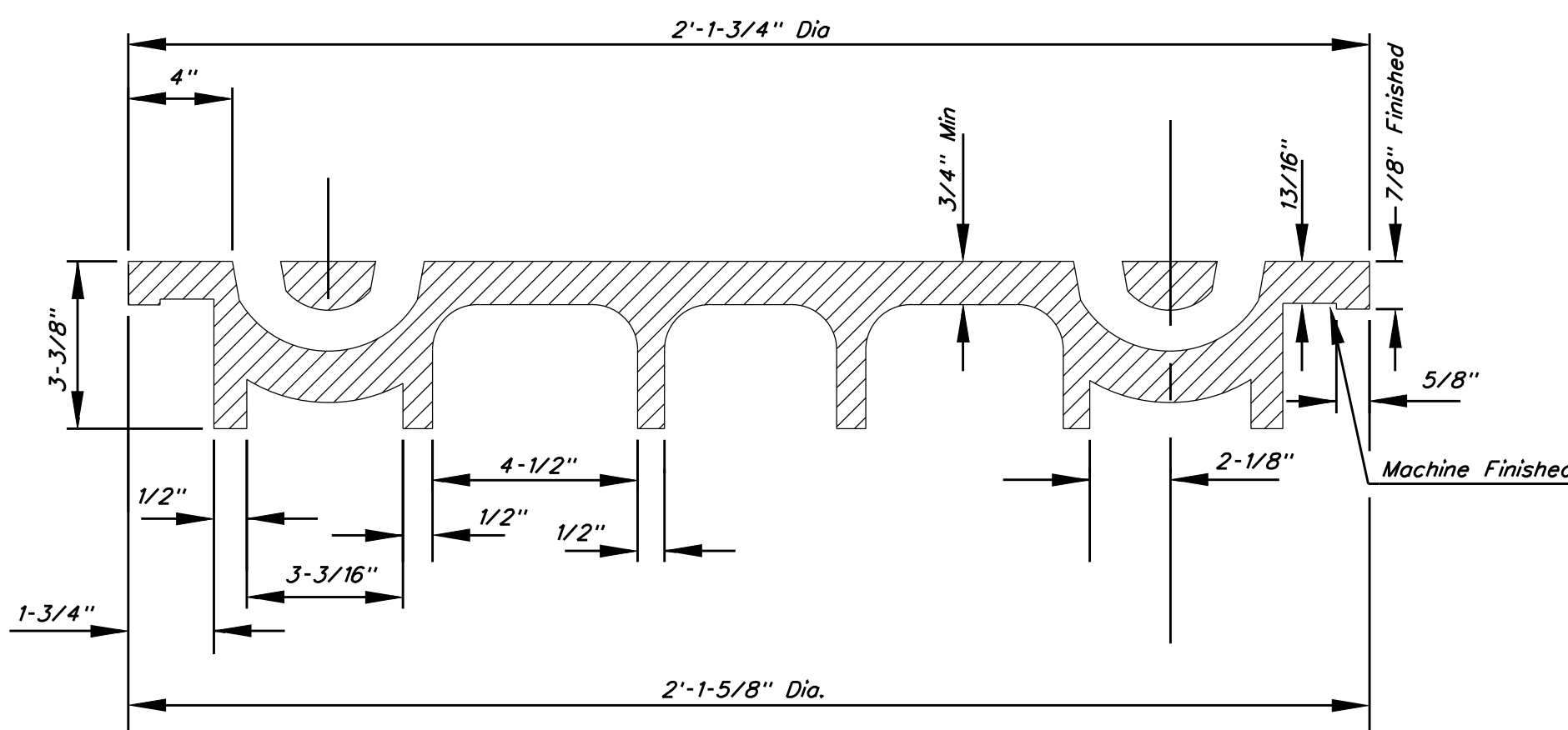
SECTION VIEW
