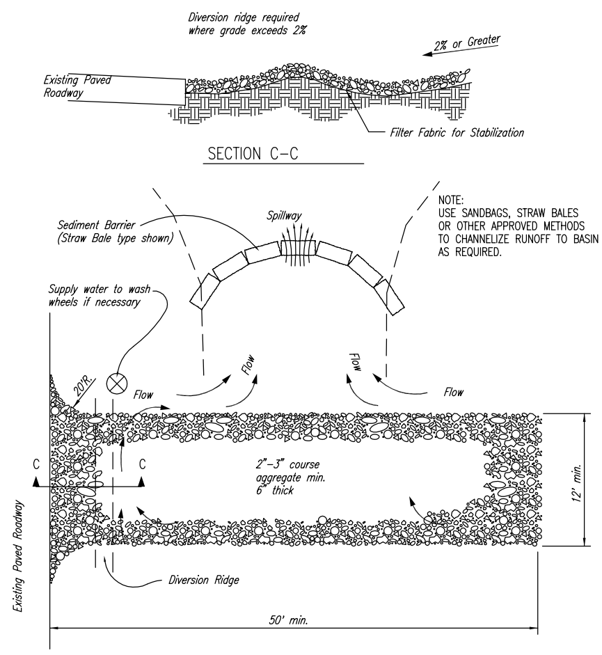
STABILIZED CONSTRUCTION ENTRANCE
