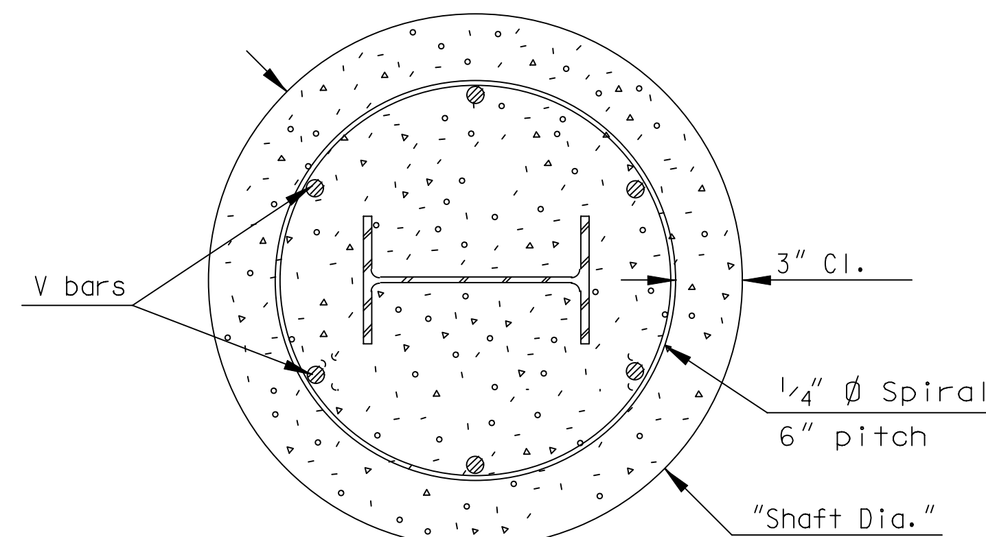
SECTION C-C
