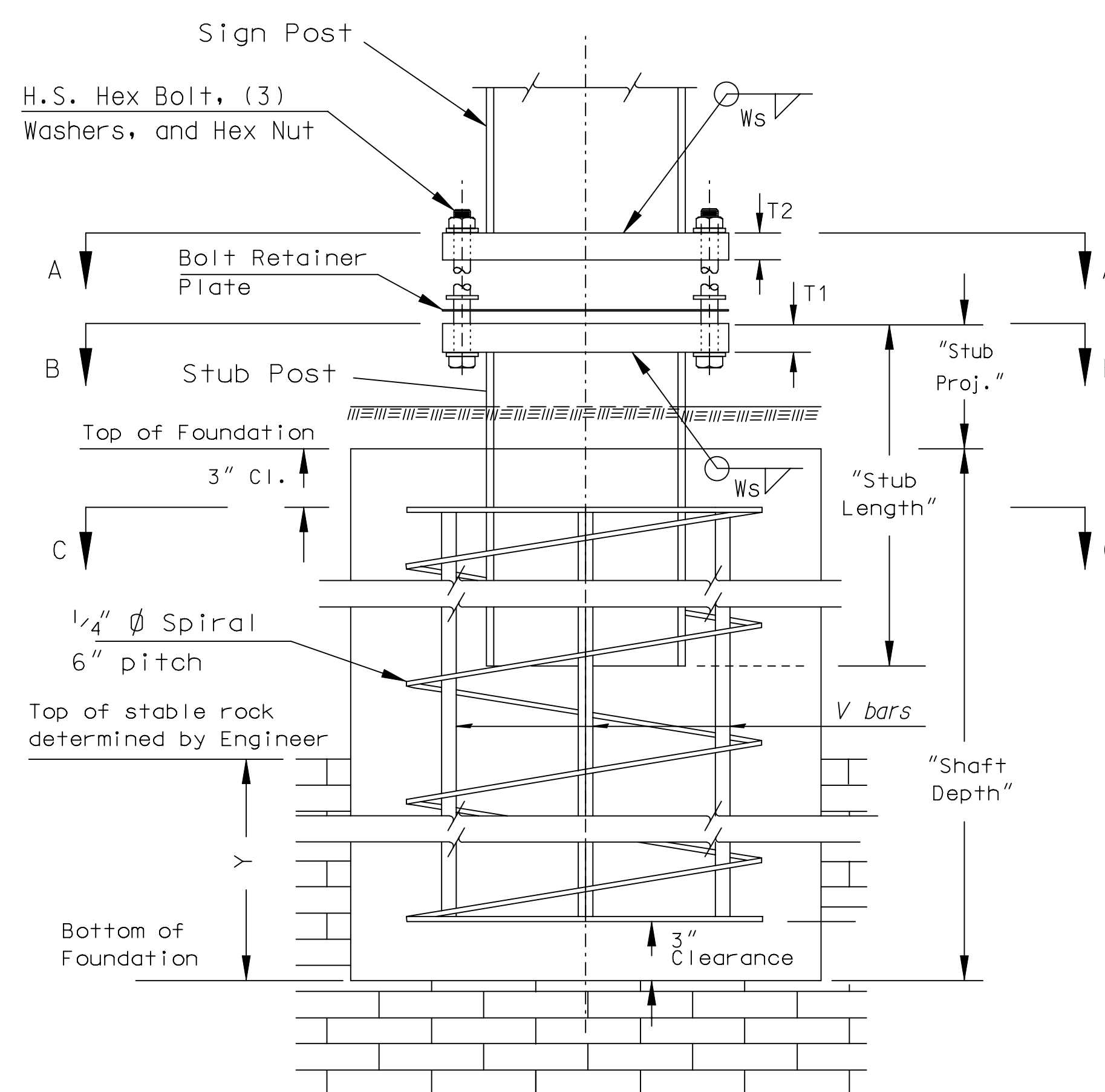
SIDE ELEVATION
