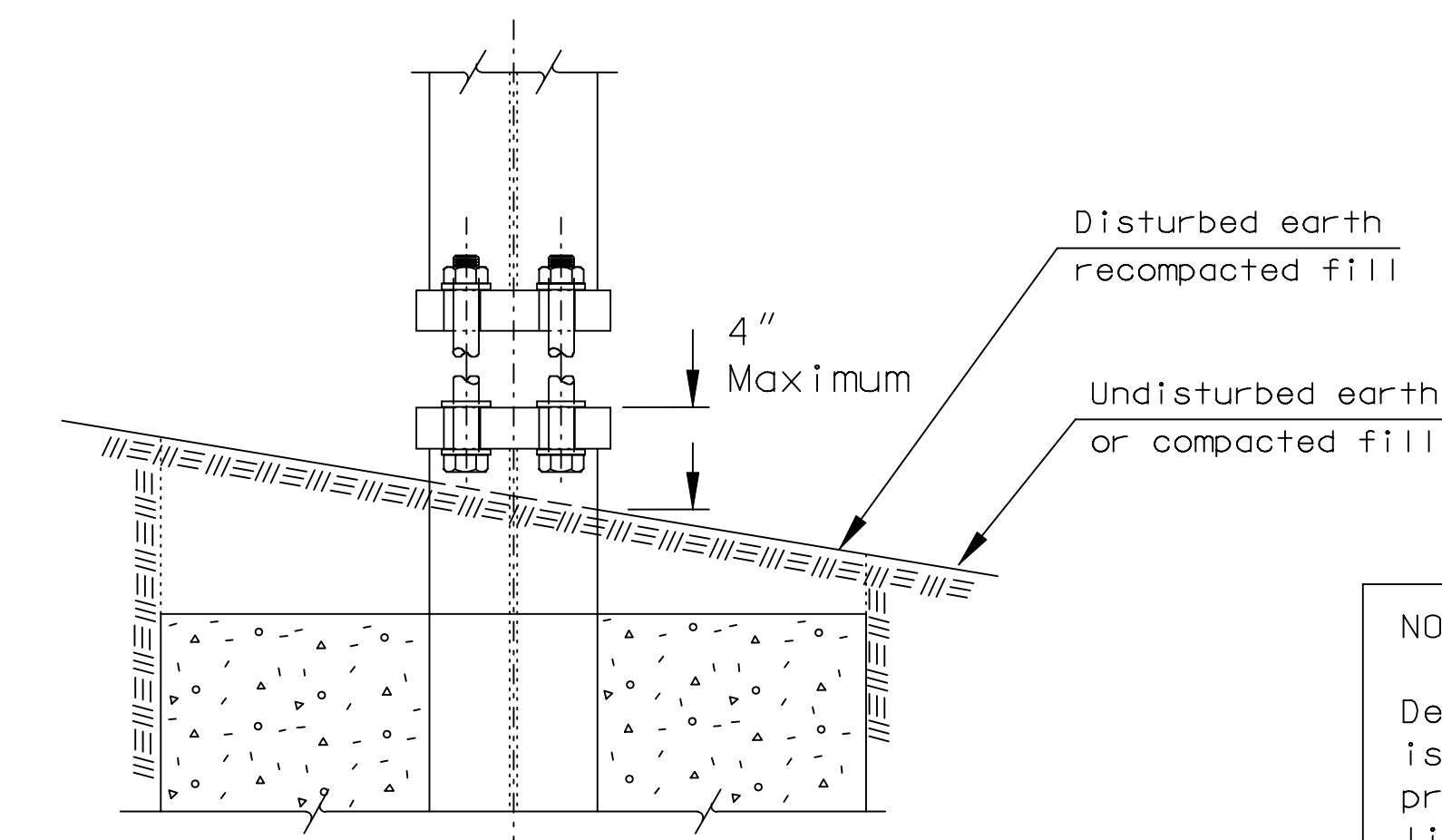
FRONT ELEVATION
