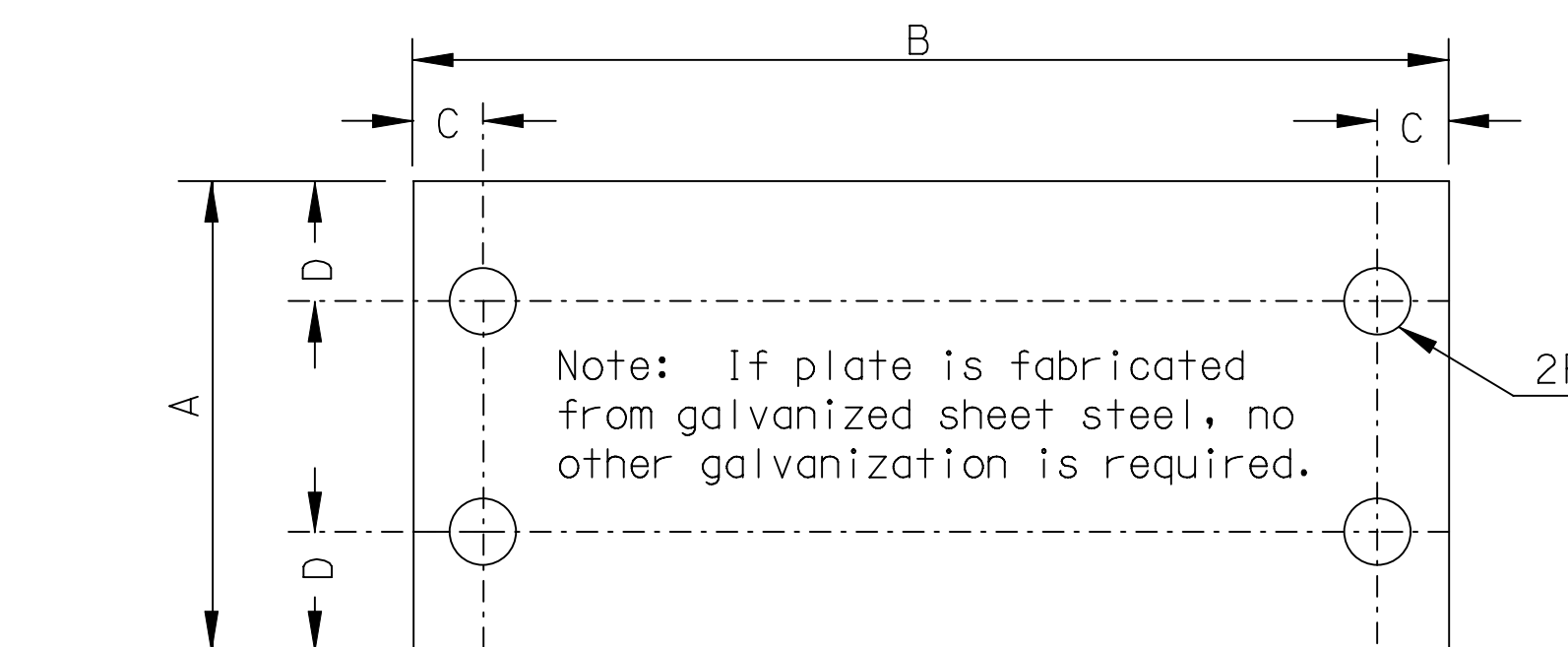
BOLT RETAINER PLATE DETAIL 30 gage sheet steel
