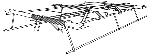
PERSPECTIVE VIEW
