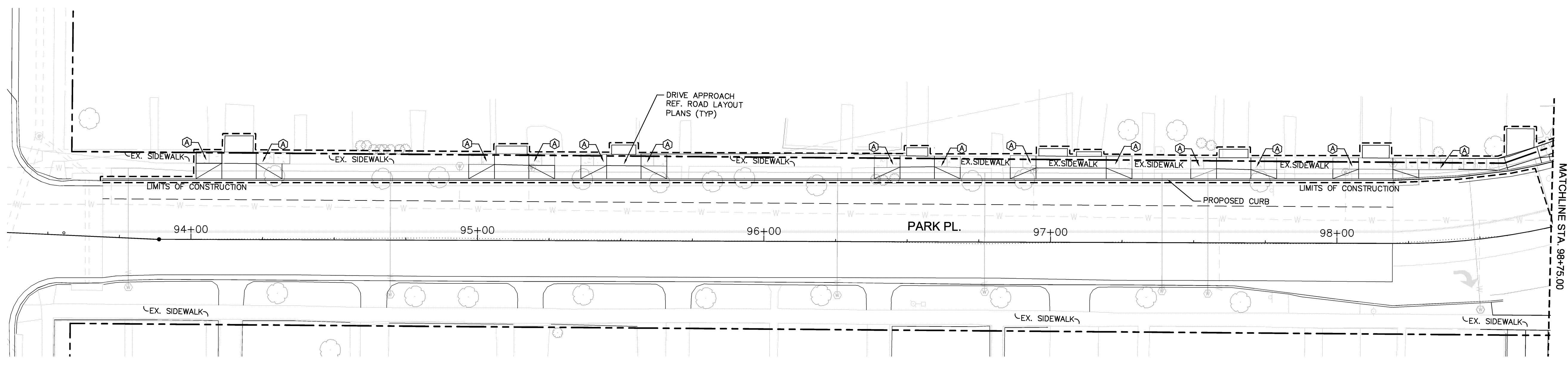
B STREETSCAPE IMPROVEMENT PLAN STA. 94+00.00 - STA. 98+75.00 (PARK PL - SOUTH OF 21ST) 1"=20'-0"
