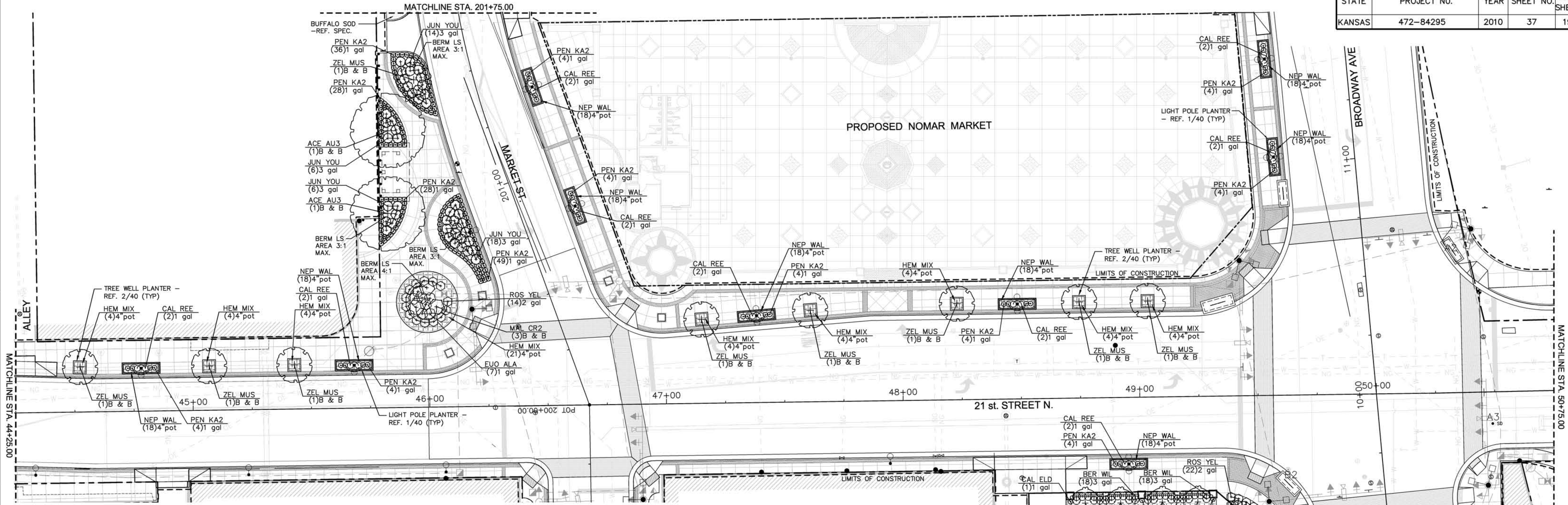
A 21ST. LANDSCAPE PLANTING PLAN 1"=20'-0" NORTH
