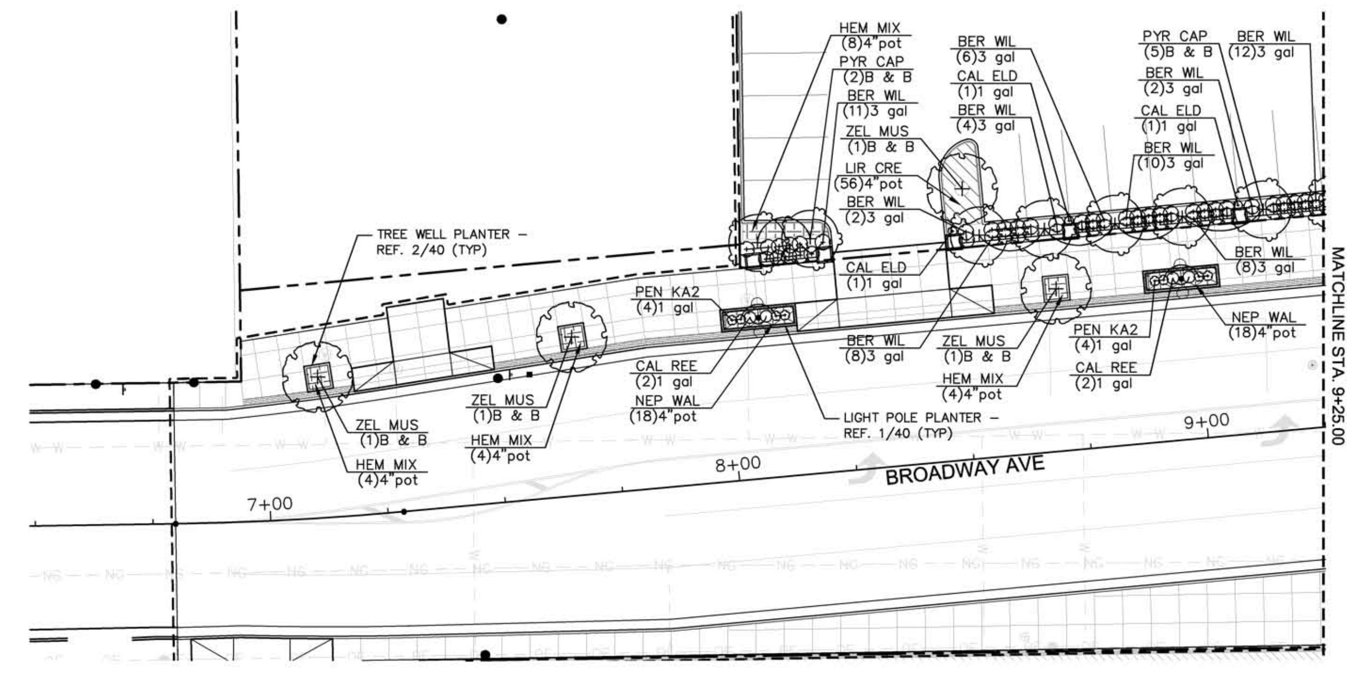
B 21ST. LANDSCAPE PLANTING PLAN BROADWAY - SOUTH OF 21ST 1"=20'-0" NORTH
