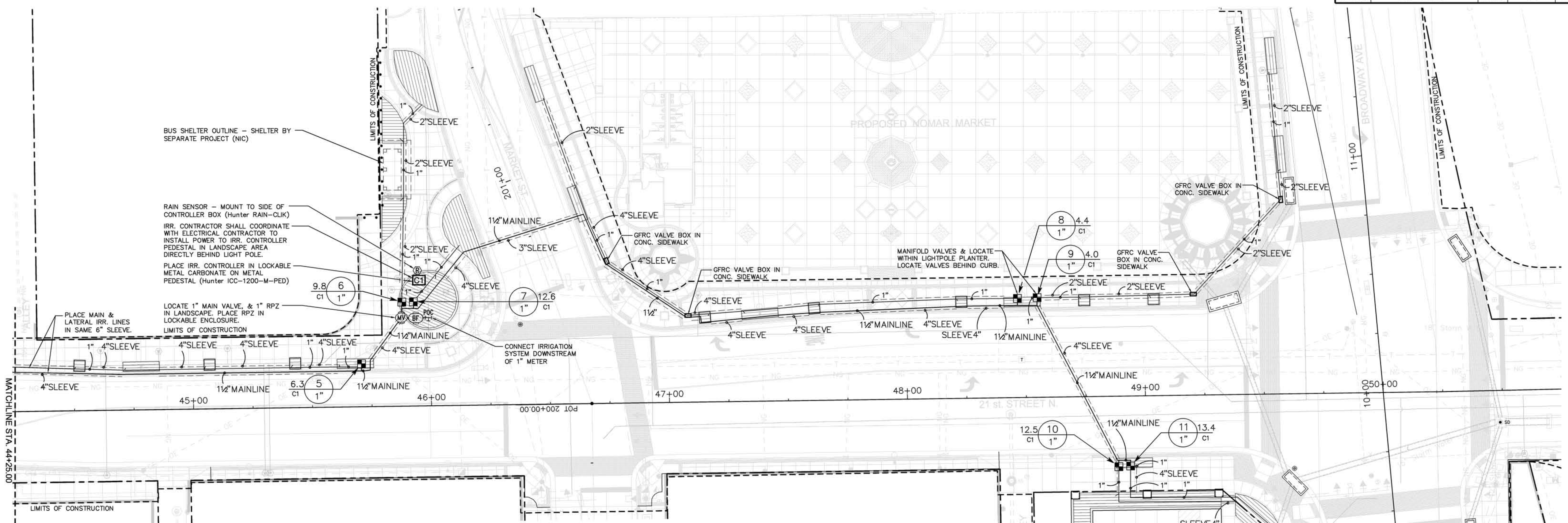
A 21ST. LANDSCAPE PLANTING PLAN STA. 44+25 TO STA. 9+25 1"=20'-0" NORTH
