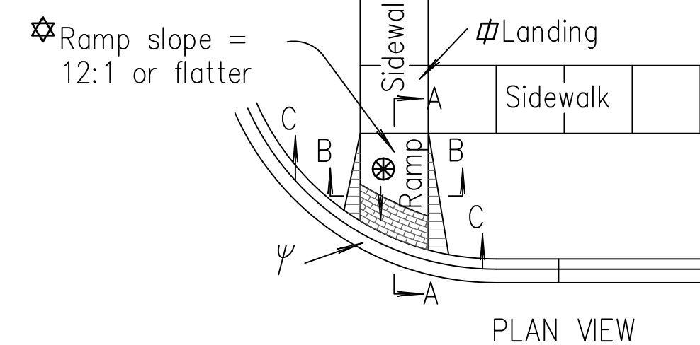
PLAN VIEW
