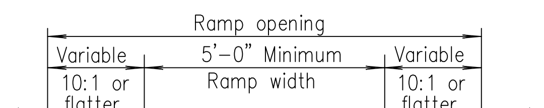
SECTION G-G
