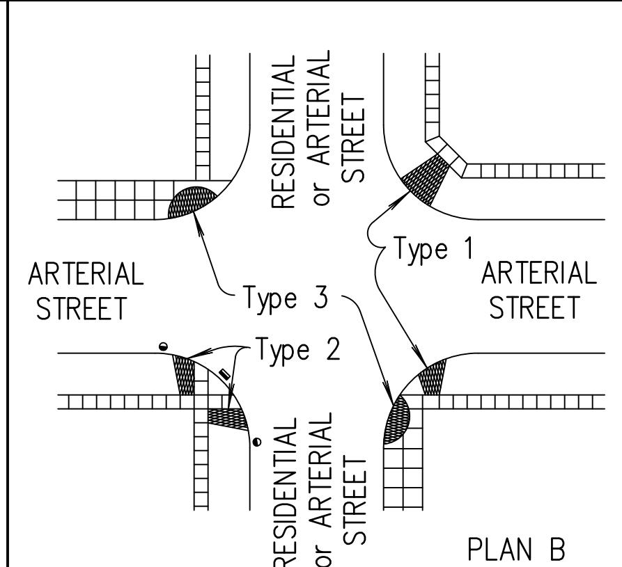
PLAN B
