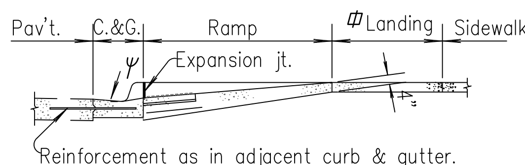
SECTION G-G
