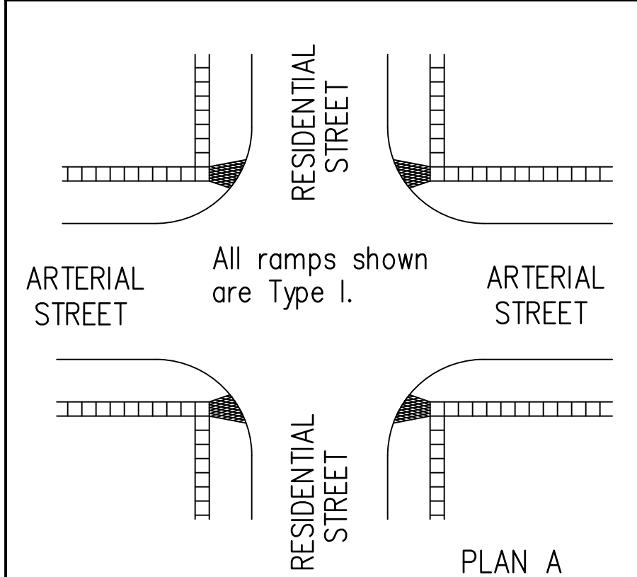
PLAN A
