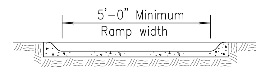
SECTION B-B
