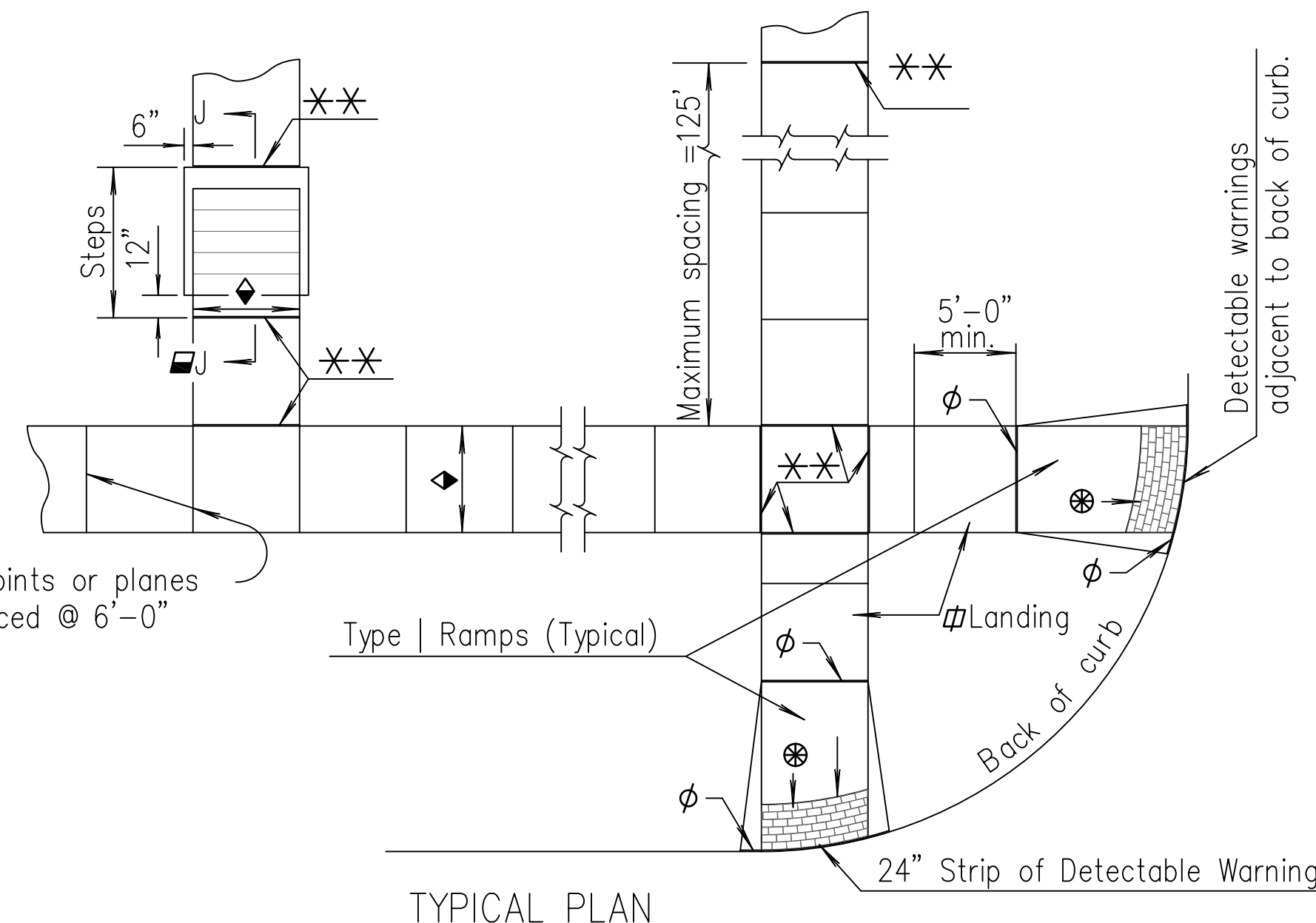
TYPICAL PLAN
