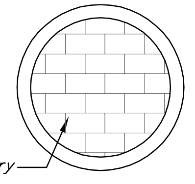
8" Brick Masonry PIPE PLUG DETAIL
