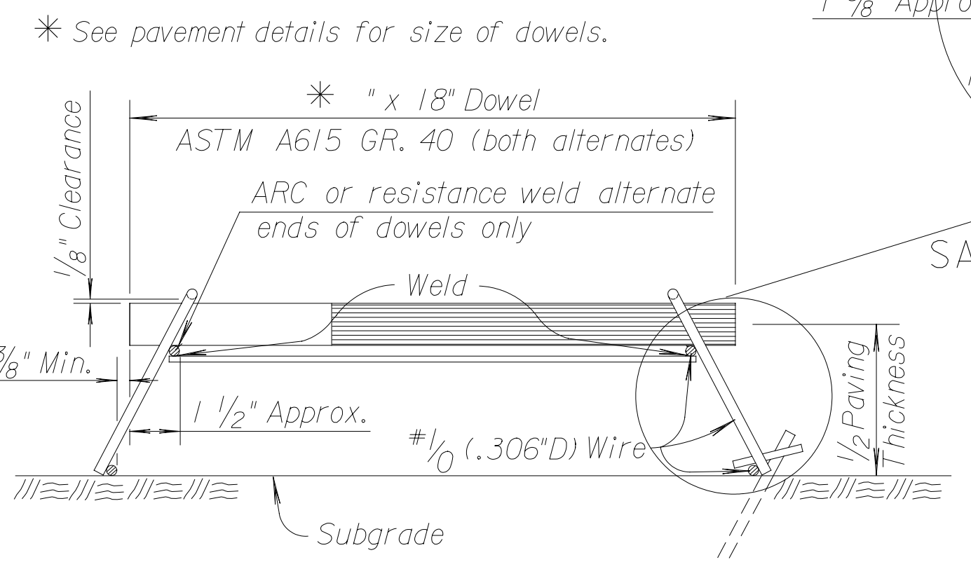
SEC. B-B
