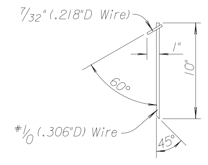
STAKE DETAIL
