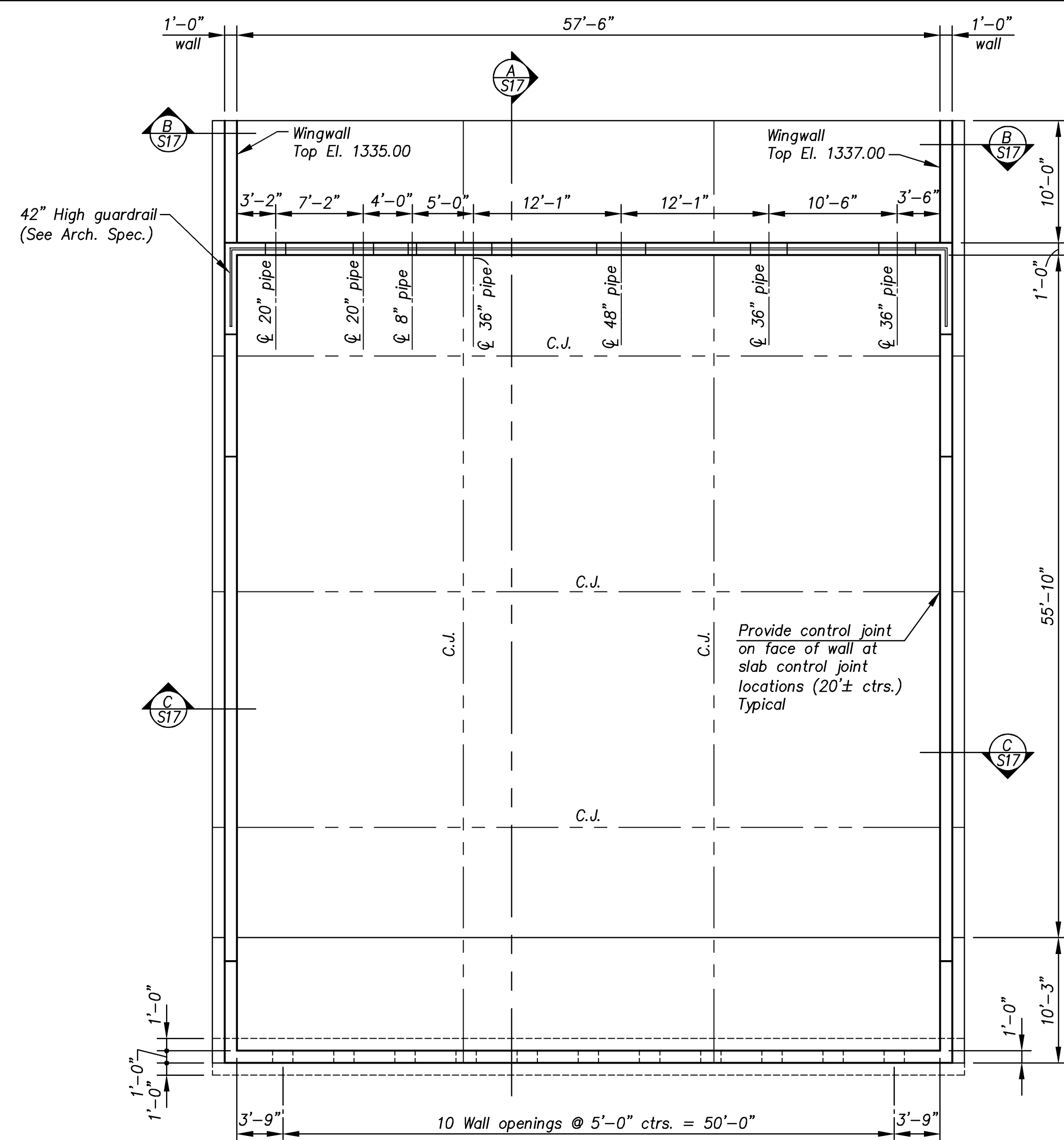
OUTFALL STRUCTURE PLAN
