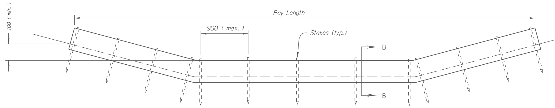
BIODEGRADABLE LOG DITCH CHECK NO SCALE
