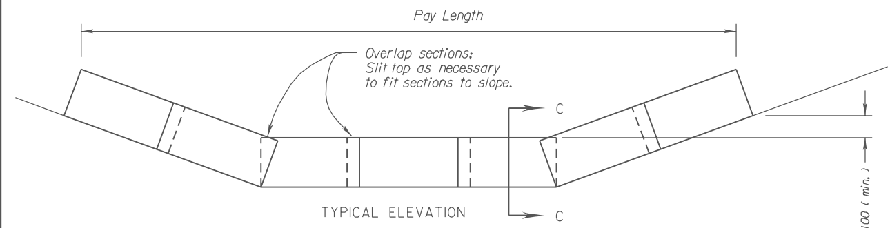
GEO-RIDGE PERMEABLE BERM DITCH CHECK NO SCALE
