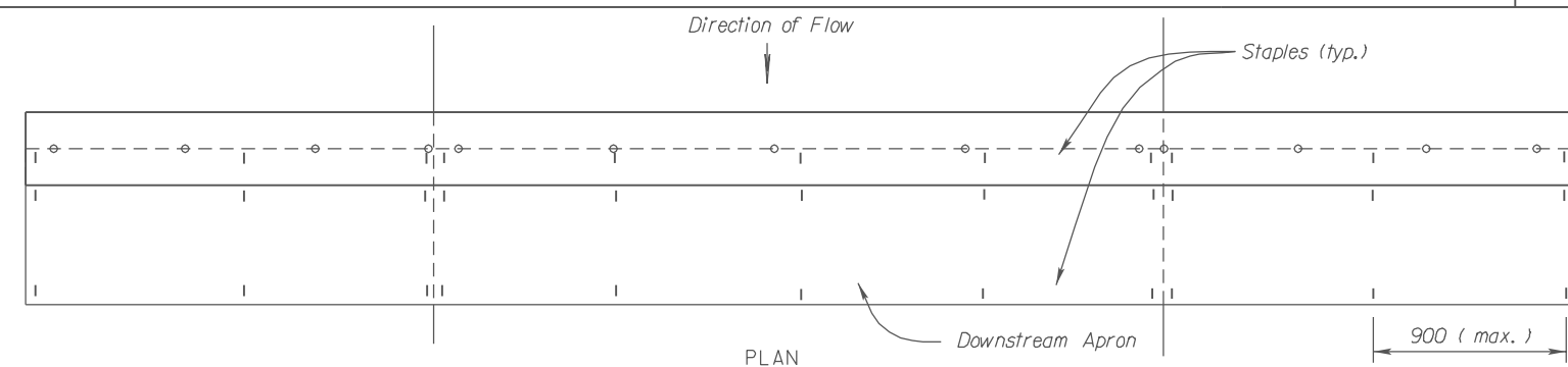
GEO-RIDGE PERMEABLE BERM DITCH CHECK NO SCALE
