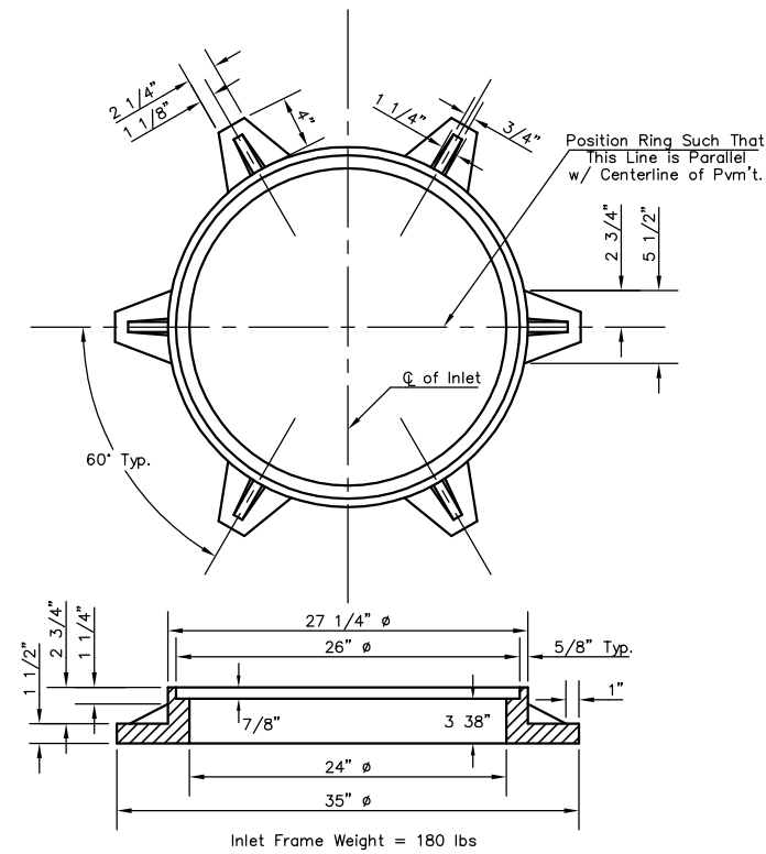
MANHOLE RING AND COVER
