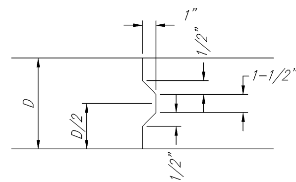
KEYWAY DETAIL
