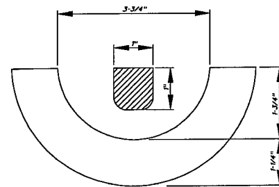
SECTION VIEW
