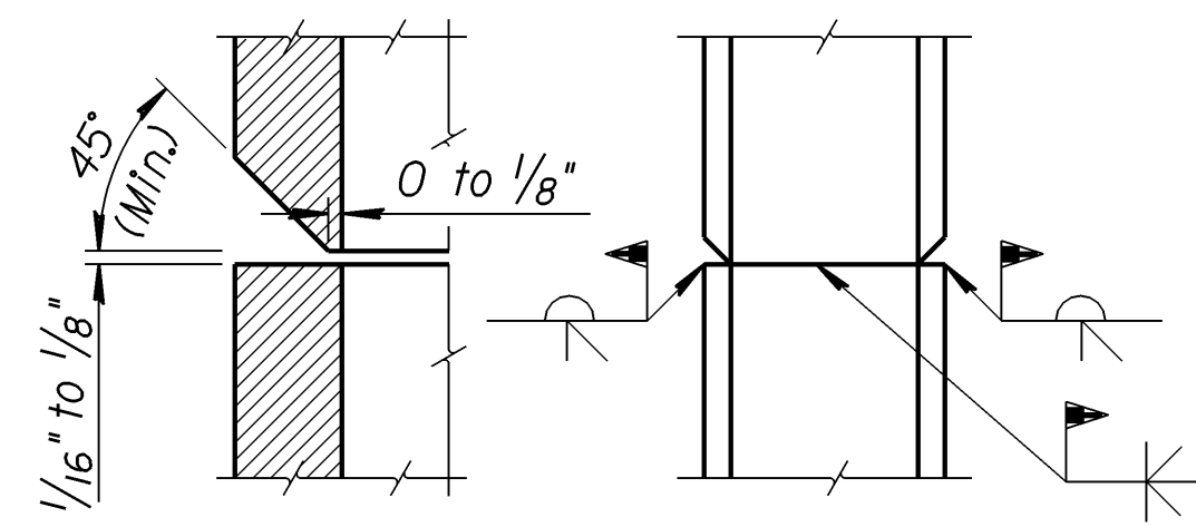
SECTION THRU FLANGE
