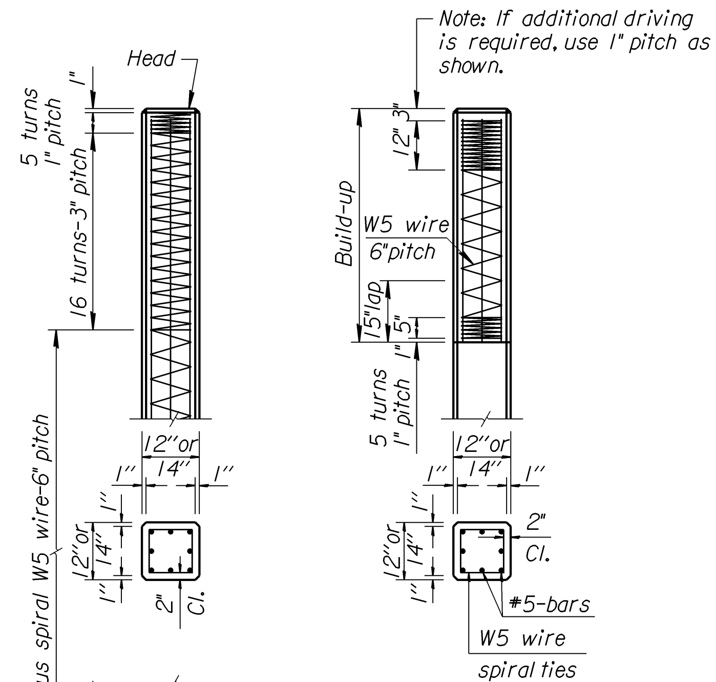
BUILD UP SECTION
