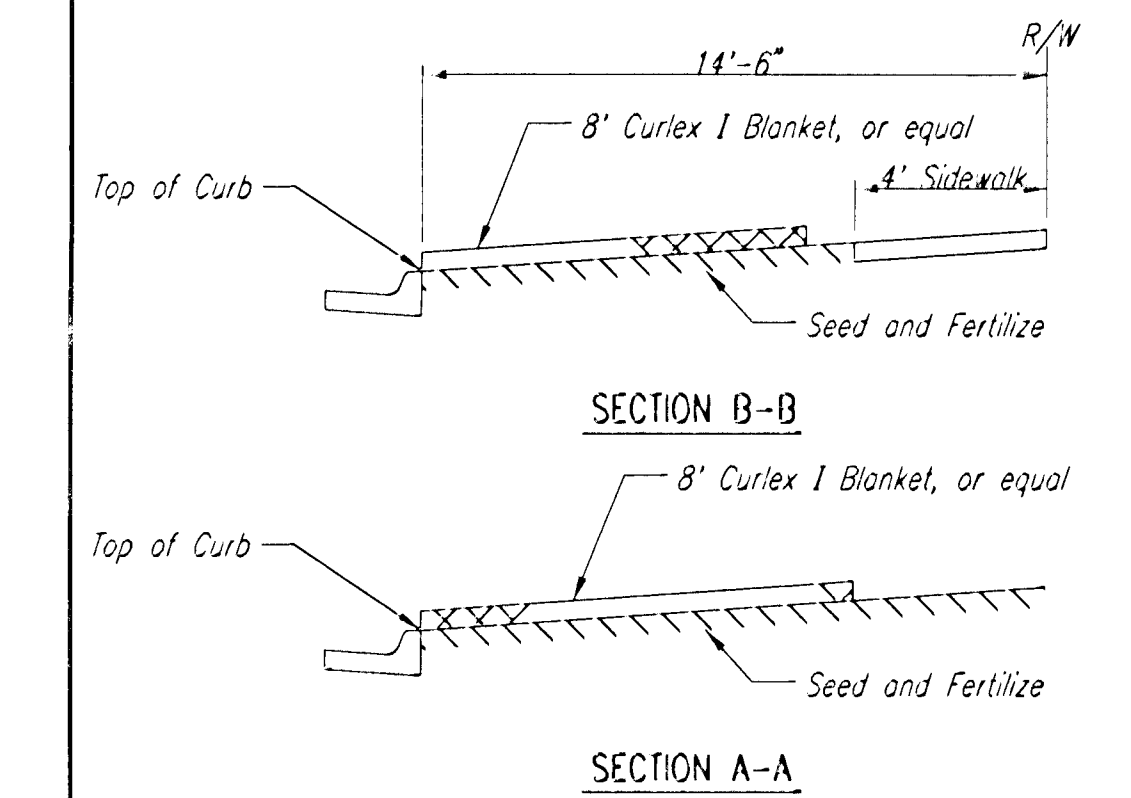
CURB BACKFILL DETAIL
