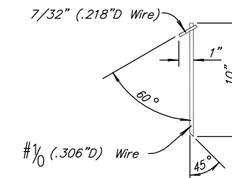
STAKE DETAIL
